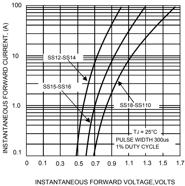
FIG.3-TYPICAL FORWARD CHARACTERISTICS
