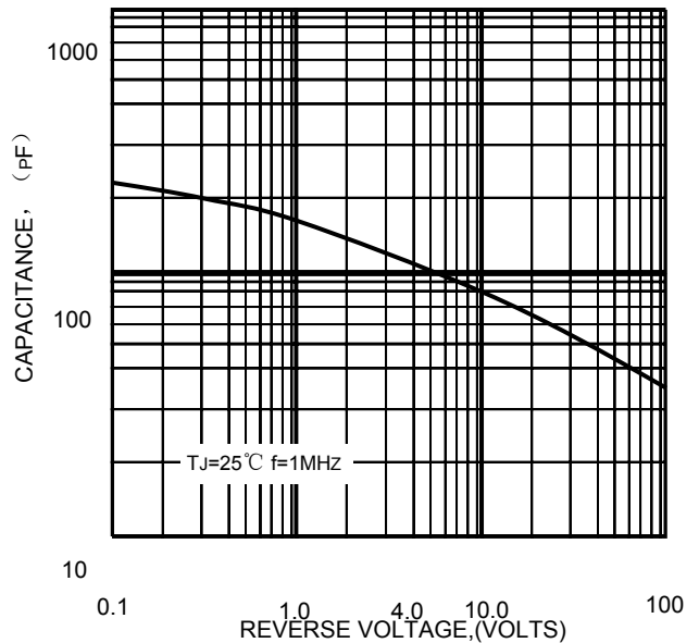
FIG.4-TYPICAL JUNCTION CAPACITANCE
