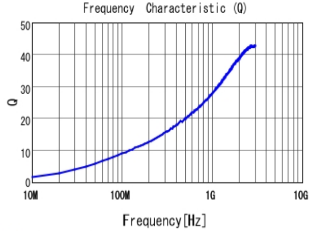
■ LQP03TN3N3C02 Q
