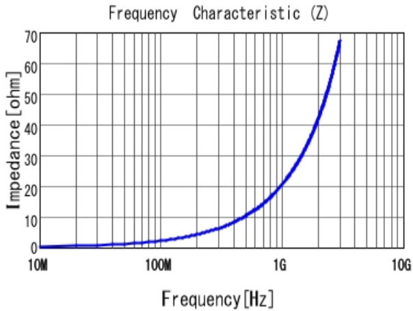
■ LQP03TN3N3C02 |Z|
