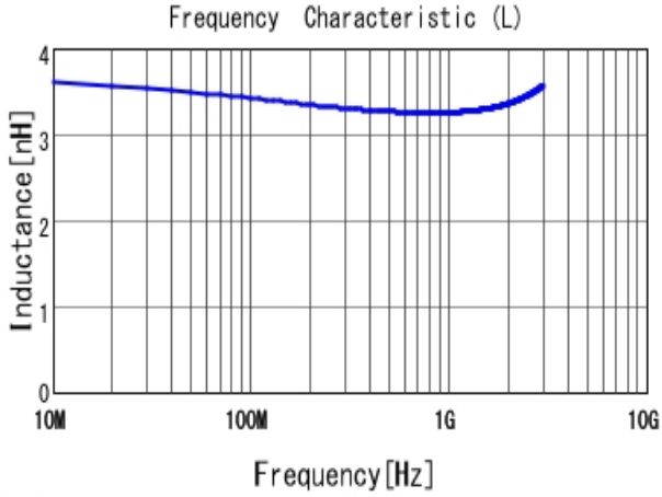
■ LQP03TN3N3C02 L
