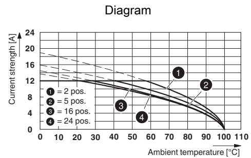
Type: MSTB 2,5/...-ST with MSTBV 2,5/...-G
