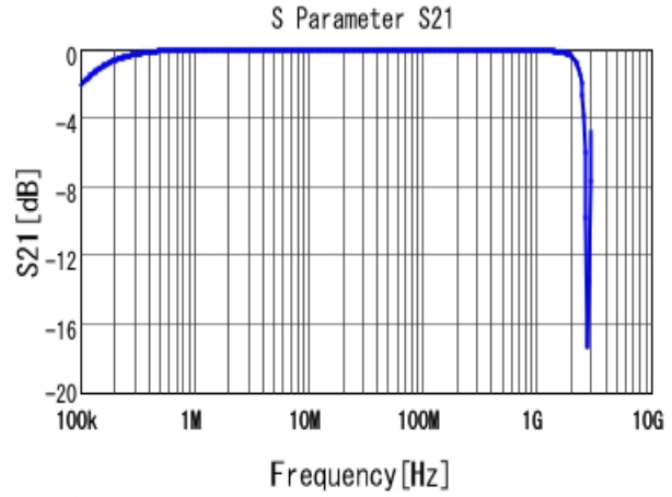
■ KRM55T7U3A203KDL1 S21 DCOV, 25degC
