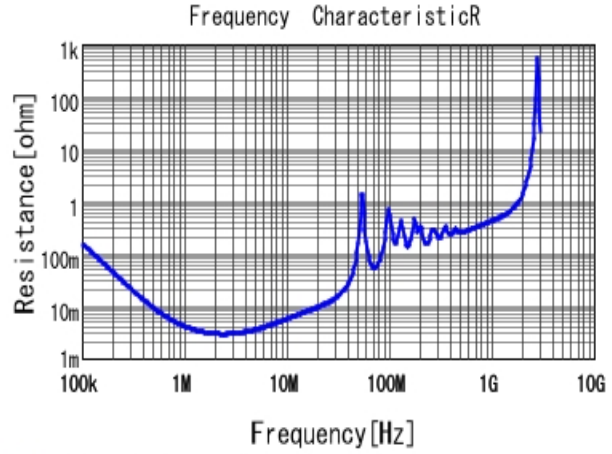
■ KRM55T7U3A203KDL1 R DC0V, 25degC
