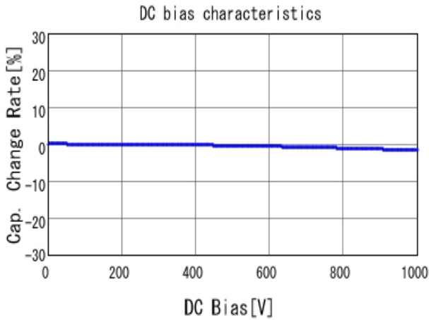
■ KRM55T7U3A203KDL1 C-DC bias capchange, 25.0degC, AC1V
