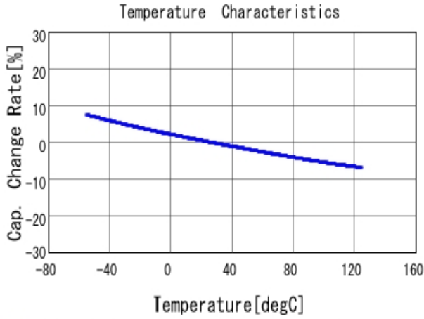
■ KRM55T7U3A203KDL1 C-Temp. capchange, DCOV, AC1Vrms
