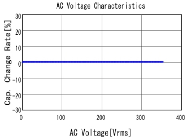
■ KRM55T7U3A203KDL1 C-AC Voltage capchange, DC0V, 25.0d
