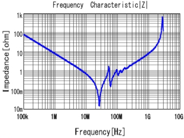
■ KRM55T7U3A203KDL1 |Z| DC0V, 25degC
