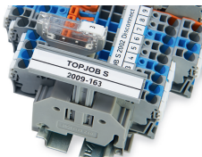
Height-adjustable group marker carrier (2009-163) for WMB markers or marking strips (2009-110)
