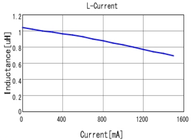
■ LQM31PN1R0M00 L-Current 20degC
