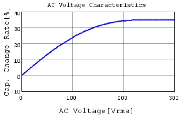
DE1E3RA102MA4BP01F C-AC Voltage capchange, I
