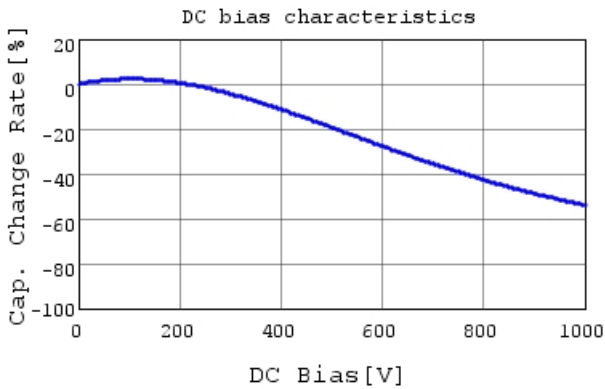
DE1E3RA102MA4BP01F C-DC bias capchange, 20.0
