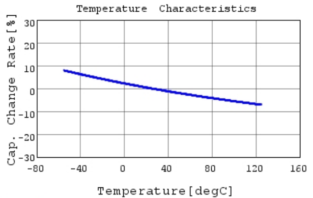
GRM31A7U3A680JW31 C-Temp. capchange, DC0V, 1
