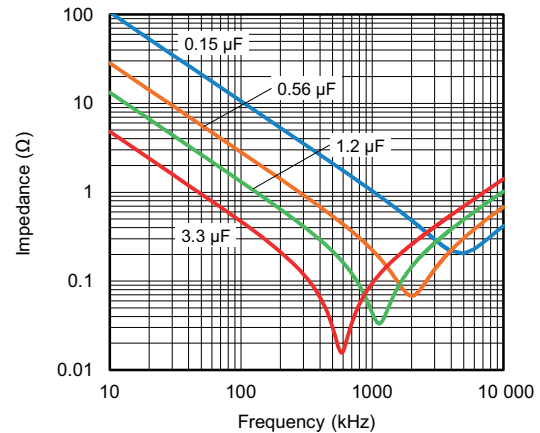
Impedance as a function of frequency (typical curve) at T_{amb} = 20\text{ }^{\circ}\text{C} (average), measurement with length 6 mm
