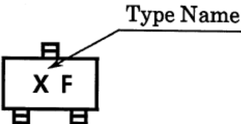
Fig. 9.6 Marking RN1106
