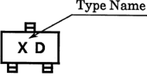
Fig. 9.4 Marking RN1104
