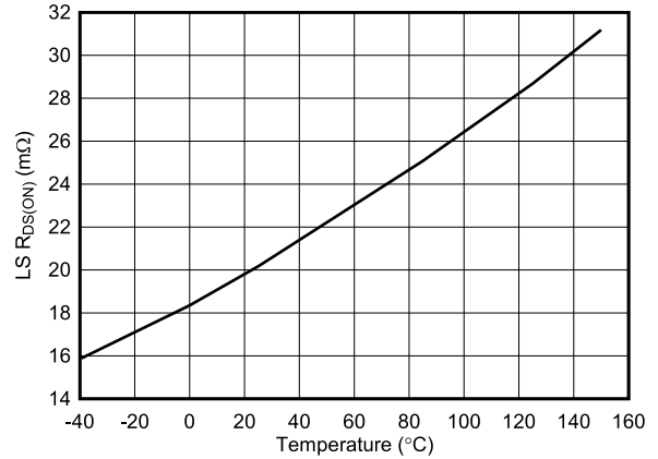
Figure 6-38. Low-Side R_{DS(ON)} vs Junction Temperature
