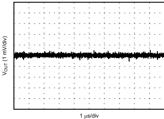
Figure 6-17. V_{OUT} Ripple after the Second L-C Filter
