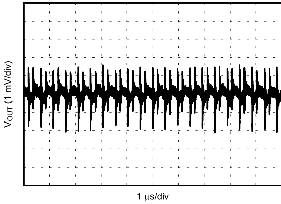
Figure 6-19. V OUT Ripple After the First L-C Filter (V OUT-Mid )
