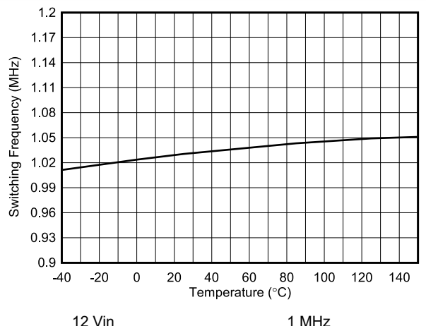
Figure 6-42. Oscillator Frequency vs Temperature
