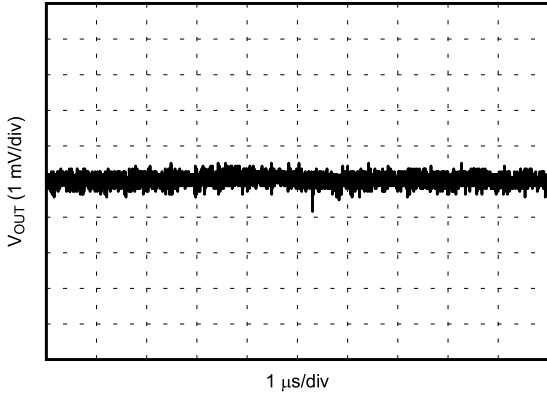
Figure 6-13. V_{OUT} Ripple After the Second L-C Filter
