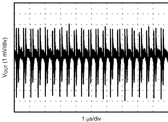
Figure 6-11. V_{OUT} Ripple After the First L-C Filter ( V_{OUT-Mid} )
