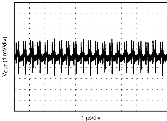
Figure 6-23. V OUT Ripple After the First L-C Filter (V OUT-Mid )
