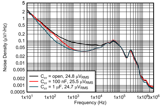
12 V to 1.8 V 2.2 \mu H, 1 MHz First L-C Only NR/SS = 470 nF, C_{FF} = Open, 100 nF, 1 \mu F
