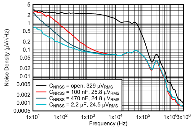
12 V to 1.8 V 2.2 \mu H, 1 MHz First L-C Only NR/SS = Open, 100 nF, 470 nF, 2.2 \mu F, BW = 100 Hz to 100 kHz
