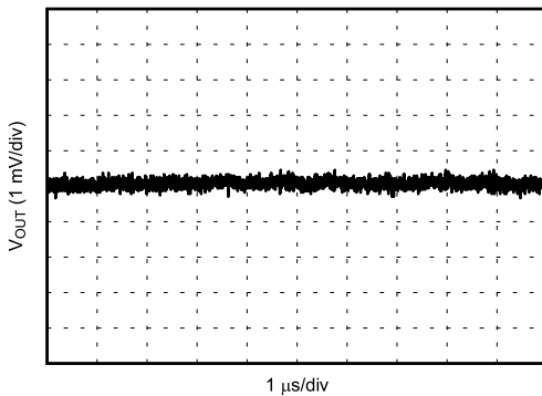
Figure 6-1. V_{OUT} Ripple After the First L-C Filter ( V_{OUT} -Mid)
