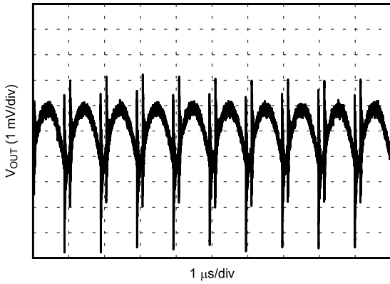
Figure 6-7. V_{OUT} Ripple After the First L-C Filter ( V_{OUT-Mid} )
