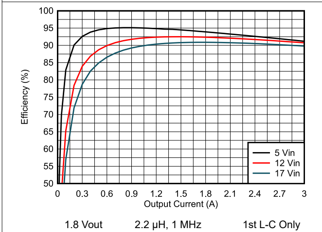
Figure 8-4. Efficiency vs Load Current
