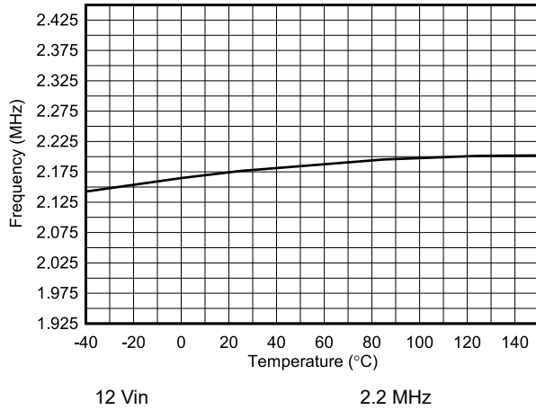
Figure 6-43. Oscillator Frequency vs Temperature
