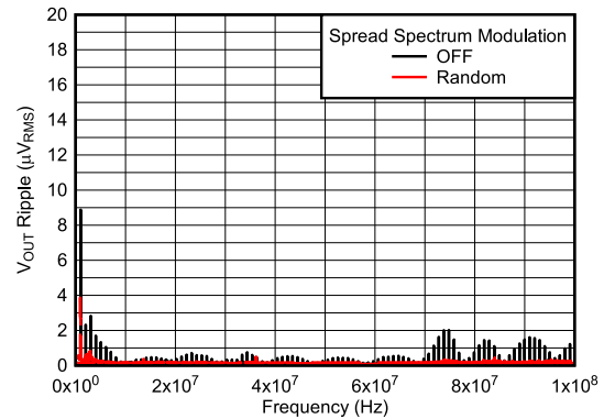
Figure 6-2. V_{OUT} Ripple FFT After the First L-C Filter ( V_{OUT} -Mid)
