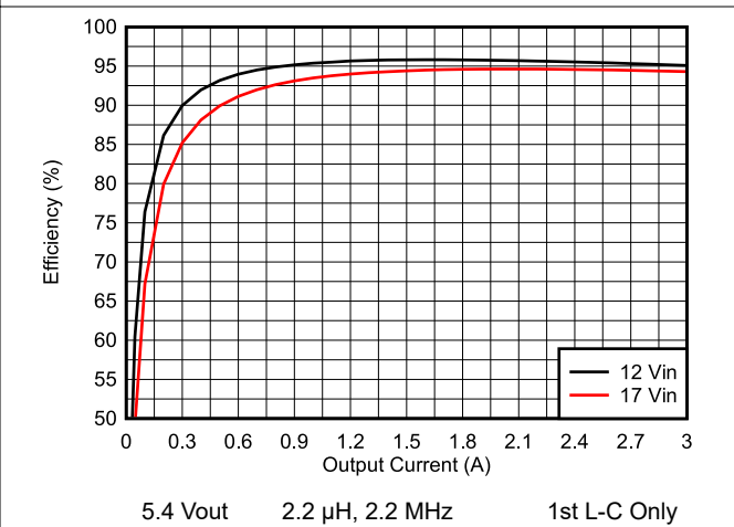
Figure 8-7. Efficiency vs Load Current
