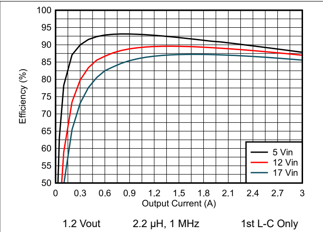
Figure 8-3. Efficiency vs Load Current
