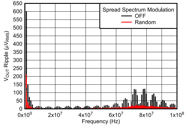
Figure 6-8. V_{OUT} Ripple FFT After the First L-C Filter ( V_{OUT-Mid} )
