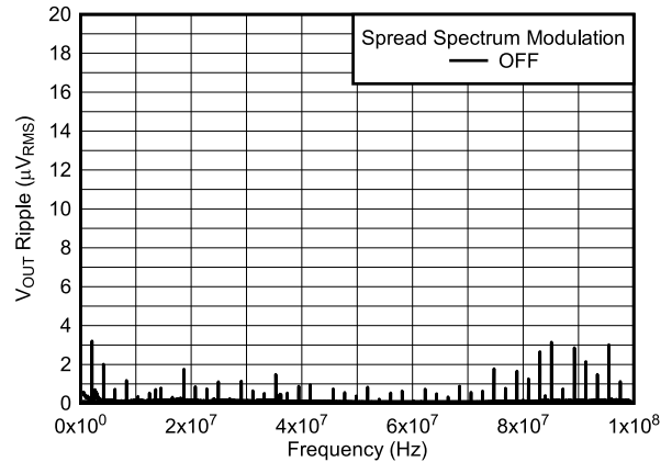
Figure 6-20. V OUT Ripple FFT After the First L-C Filter (V OUT-Mid )
