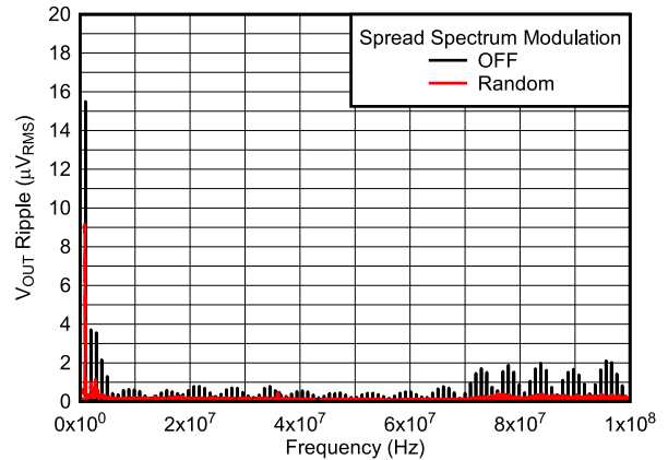
Figure 6-8. V_{OUT} Ripple FFT After the First L-C Filter ( V_{OUT-Mid} )
