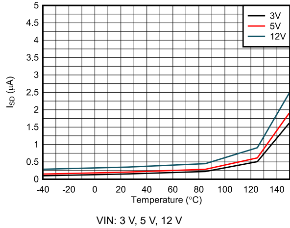
Figure 6-44. Shutdown Current vs Temperature
