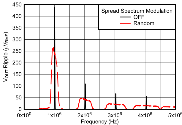
12 V to 1.2 V, 1 A 2.2 \mu H, 1 MHz S-CONF = OFF, Random
