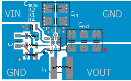
Figure 10-1. Recommended Layout for Single L-C Filter
