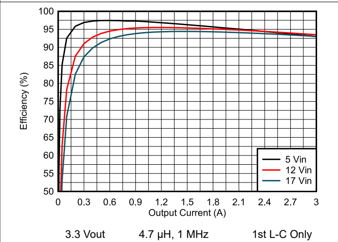
Figure 8-5. Efficiency vs Load Current
