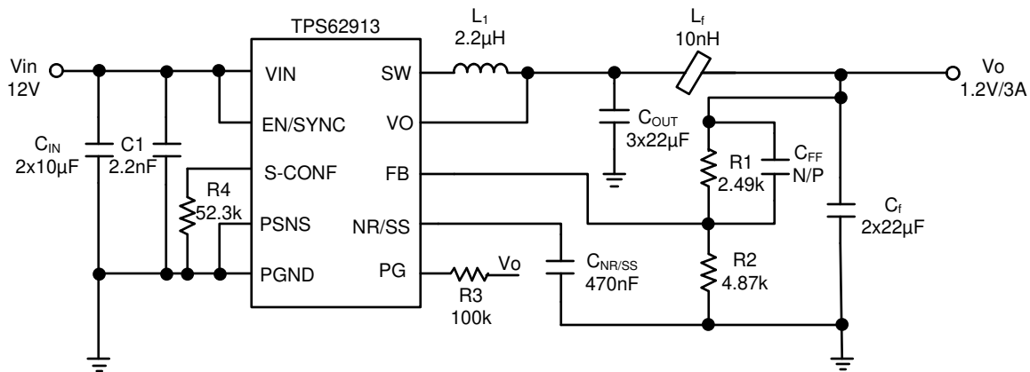
Figure 8-1. Typical Schematic
