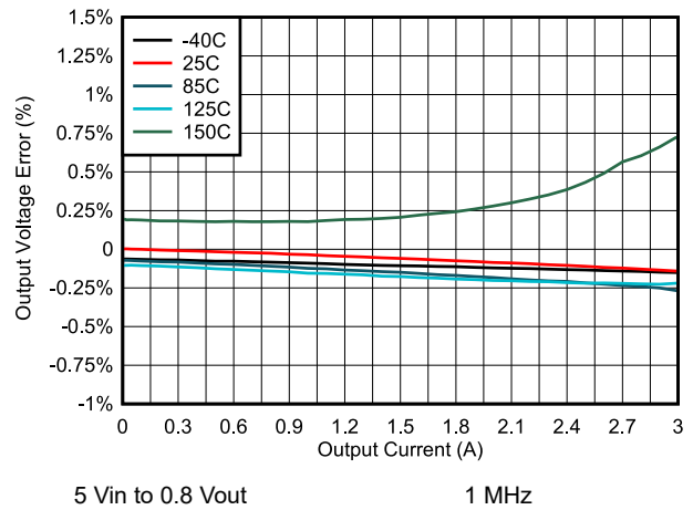
Figure 6-40. Output Voltage Error vs Load
