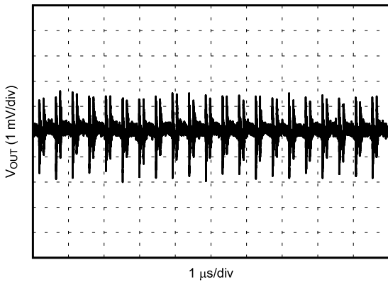
Figure 6-15. V_{OUT} Ripple After the First L-C Filter ( V_{OUT-Mid} )
