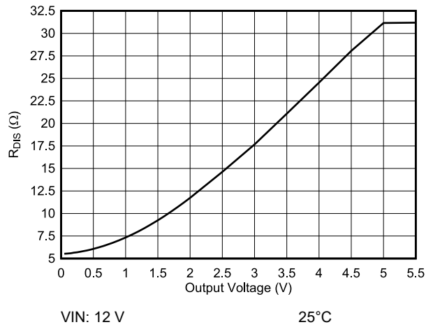
Figure 6-45. Output Discharge Resistance vs Output Voltage
