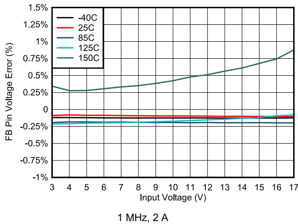
Figure 6-39. FB Pin Voltage Error vs Input Voltage
