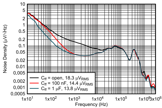
12 V to 3.3 V 2.2 \mu H, 2.2 MHz First L-C Only NR/SS = 470 nF, C_{FF} = Open, 100 nF, 1 \mu F
