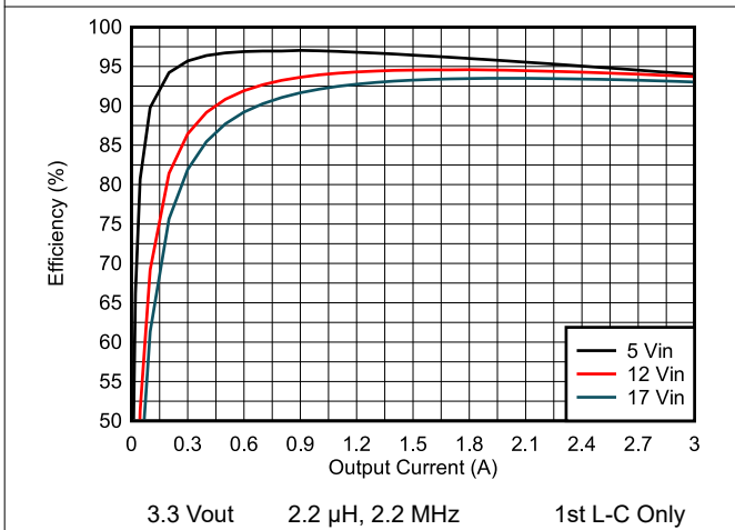
Figure 8-6. Efficiency vs Load Current
