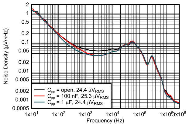
12 V to 1.2 V 2.2 \mu H, 1 MHz First L-C Only NR/SS = 470 nF, C_{FF} = Open, 100 nF, 1 \mu F
