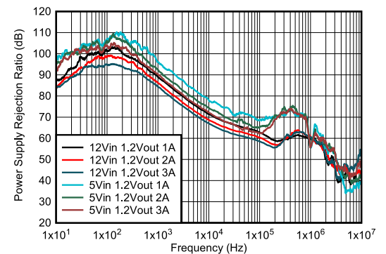
12 V to 1.2 V 2.2 \mu H, 1 MHz First L-C Only 1 A, 2 A, 3 A
