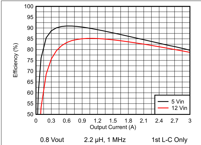
Figure 8-2. Efficiency vs Load Current
