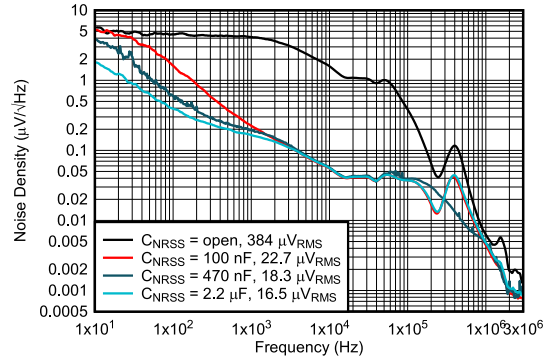
12 V to 3.3 V 2.2 \mu H, 2.2 MHz First L-C Only NR/SS = Open, 100 nF, 470 nF, 2.2 \mu F, BW = 100 Hz to 100 kHz
