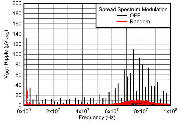
Figure 6-20. V OUT Ripple FFT After the First L-C Filter (V OUT-Mid )
