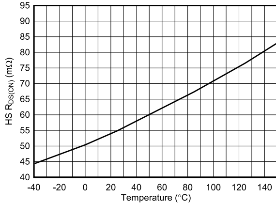
Figure 6-37. High-Side R_{DS(ON)} vs Junction Temperature
