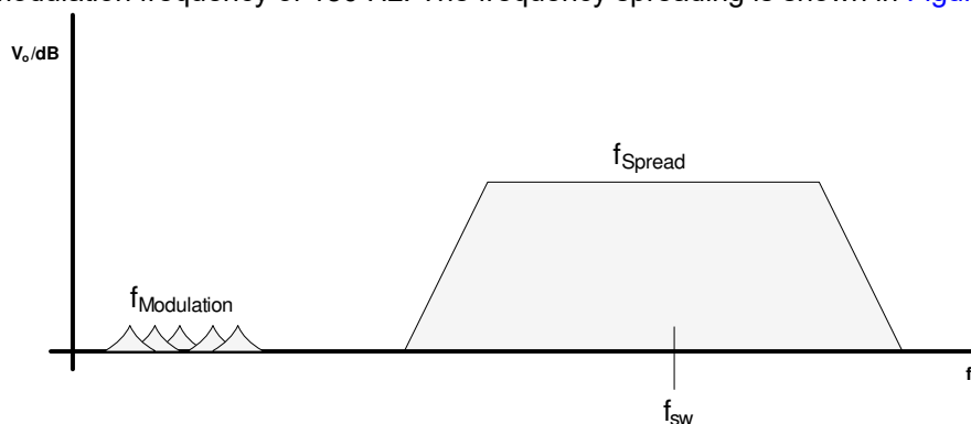
Figure 7-2. Randomized Spread Spectrum Modulation
