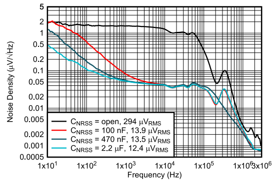
5 V to 1.2 V 2.2 \mu H, 2.2 MHz First L-C Only NR/SS = Open, 100 nF, 470 nF, 2.2 \mu F, BW = 100 Hz to 100 kHz
