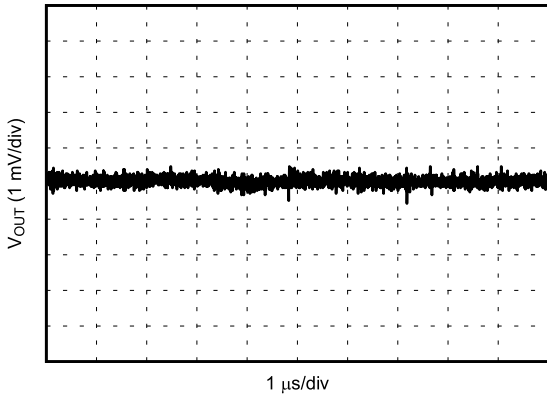
5 V to 3.3 V, 1 A 2.2 \mu H, 2.2 MHz First and second L-C
