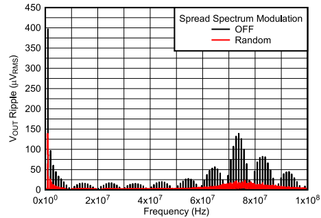
Figure 6-2. V_{OUT} Ripple FFT After the First L-C Filter ( V_{OUT} -Mid)
