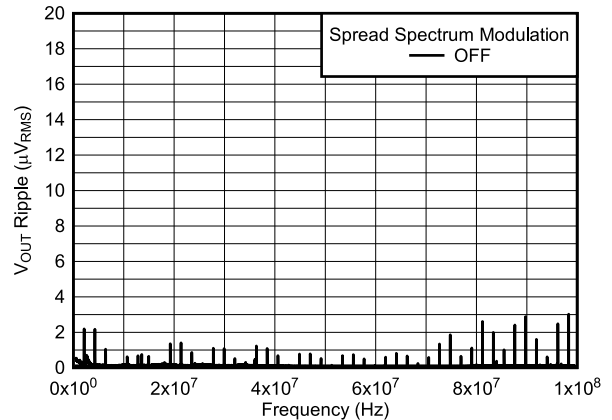
Figure 6-16. V_{OUT} Ripple FFT After the First L-C Filter ( V_{OUT-Mid} )
