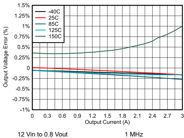
Figure 6-41. Output Voltage Error vs Load
