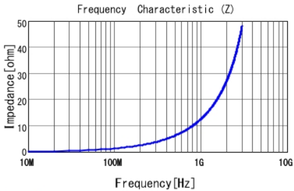
LQG15HH2N0S02 |Z|
