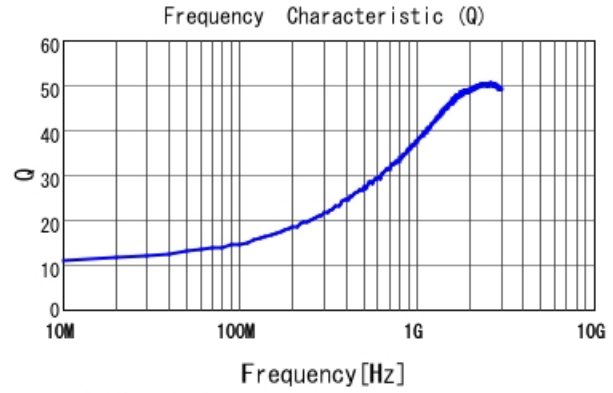
LQG15HH2N0S02 Q
