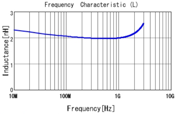
LQG15HH2N0S02 L
