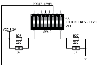
Figure 6-2: Tri-state DIP switch on PORTF
