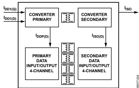
Figure 29. Power Consumption Within the ADuM5401/ADuM5402/ADuM5403/ADuM5404
