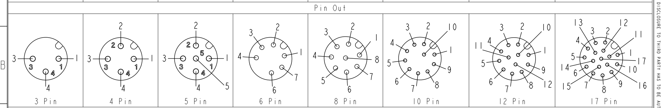
Pin Assignments Front View
