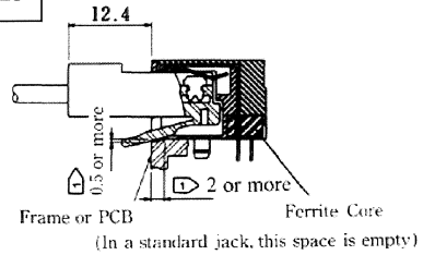
View of mating plug A-A
