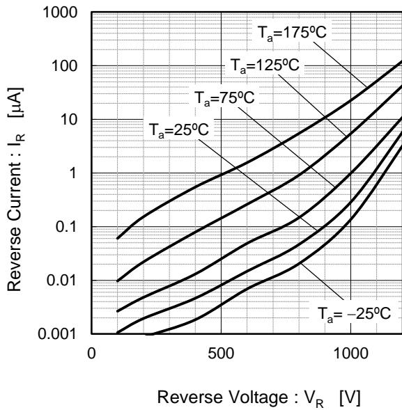
Fig.3 V_R - I_R Characteristics (Per Leg)
