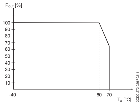
Fig. 5 Derating
