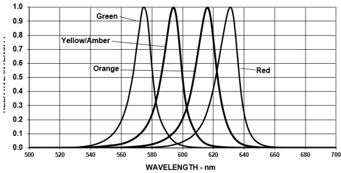
Figure 1: Relative Intensity versus Wavelength
