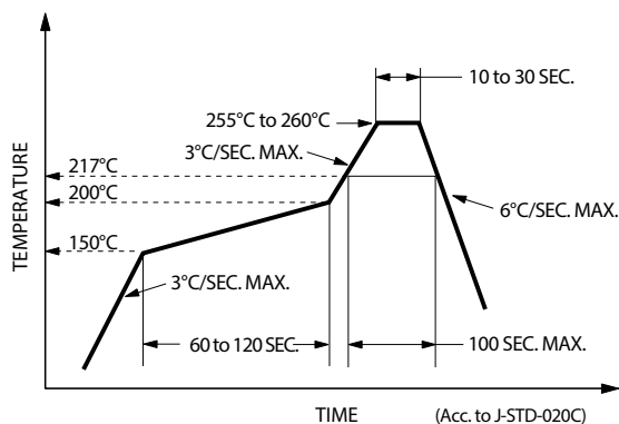
Figure 13: Recommended Lead-Free Reflow Soldering Profile
