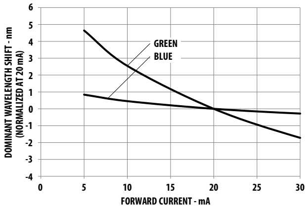
Figure 6 Dominant Wavelength Shift vs. Forward Current
