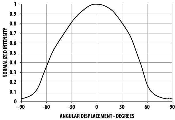
Figure 7 Radiation Pattern for Major Axis
