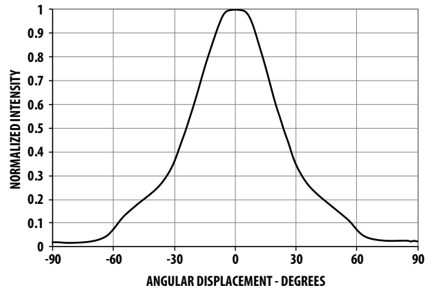
Figure 8 Radiation Pattern for Minor Axis
