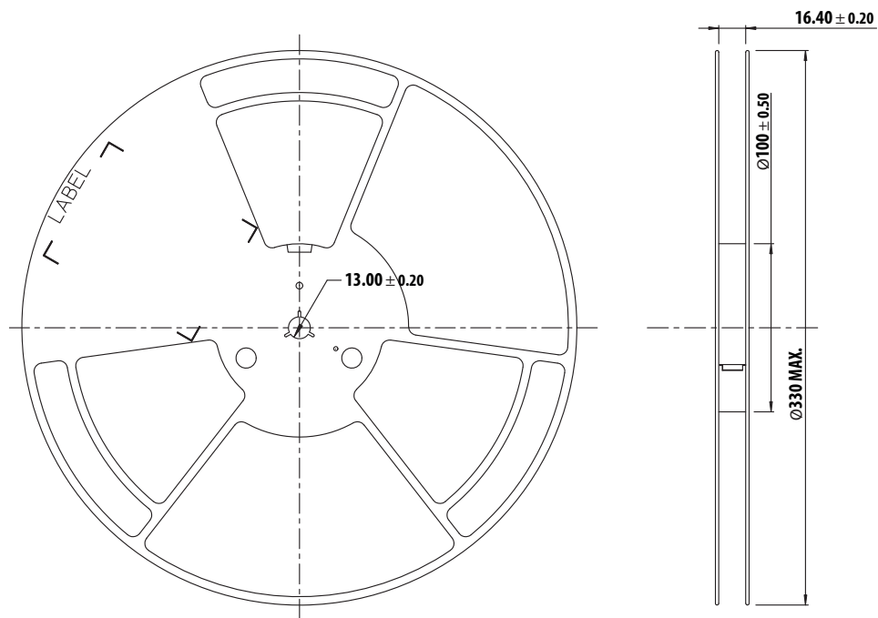
Figure 13 Reel Dimension
