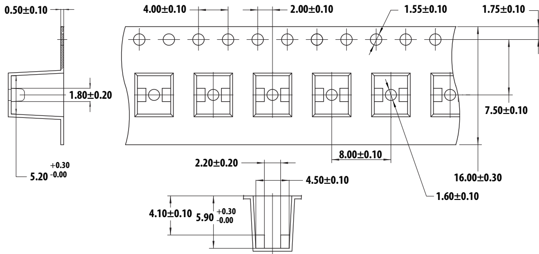
Figure 12 Carrier Tape Dimension
