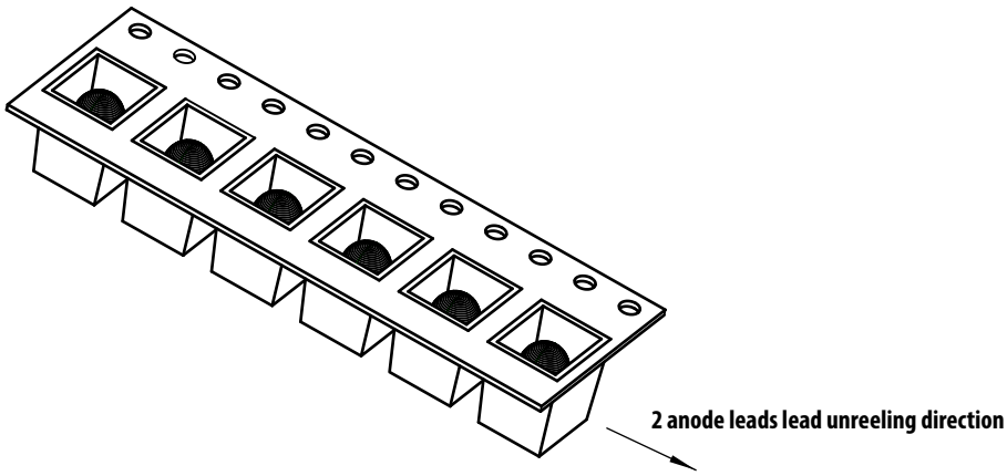
Figure 14 Unit Orientation from Reel
