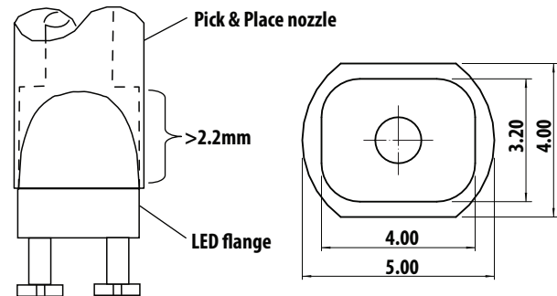
Figure 18 Nozzle Diagram
