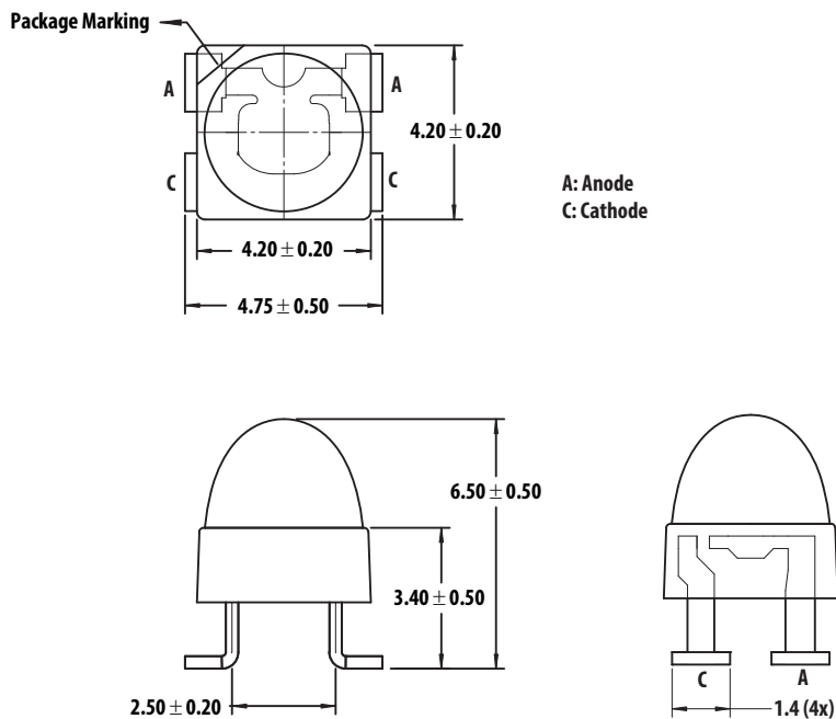
Figure 1: Package Dimensions
