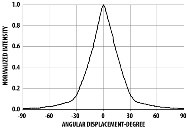
Figure 12: Radiation Pattern for X Axis
