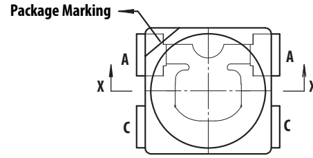
Figure 13: Component Axis for Radiation Pattern
