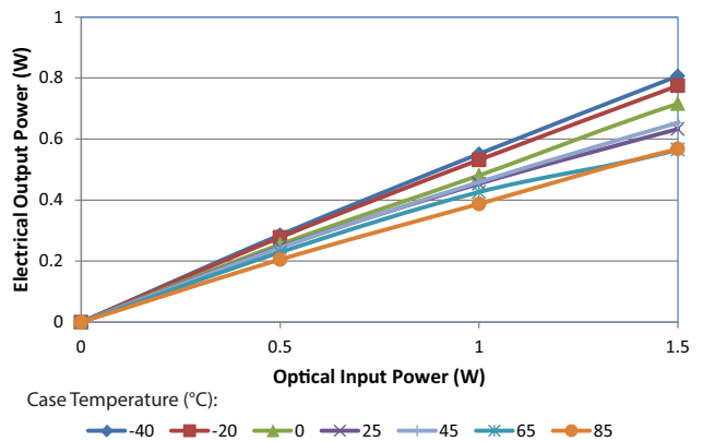
Figure 6: Electrical Output Power; 1 × AFBR-POCx04L
