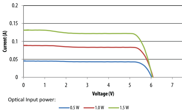
Figure 11: Output I-V Curves at 85°C; 1 × AFBR-POCx06L
