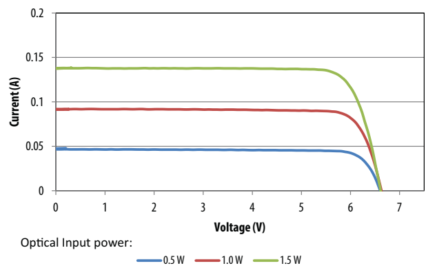
Figure 10: Output I-V Curves at 25°C; 1 × AFBR-POCx06L
