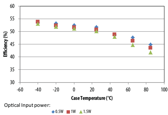
Figure 13: Efficiency; 1 × AFBR-POCx06L
