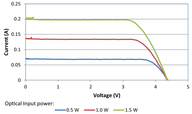
Figure 4: Output I-V Curves at 25°C; 1 × AFBR-POCx04L
