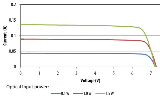
Figure 9: Output I-V Curves at -40°C; 1 × AFBR-POCx06L
