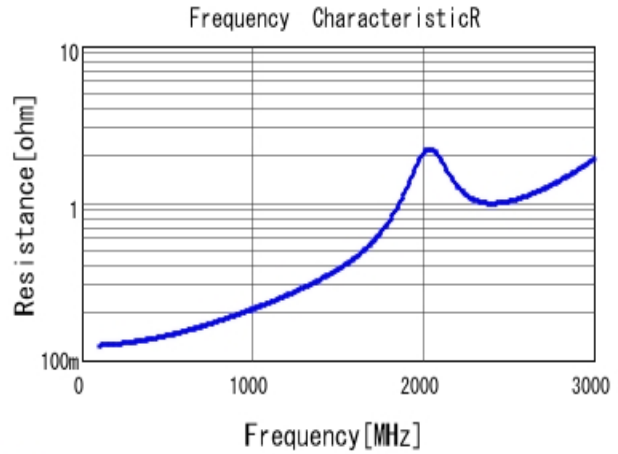
■ GRM31A5C3A820JW01 R DC0V, 25degC
