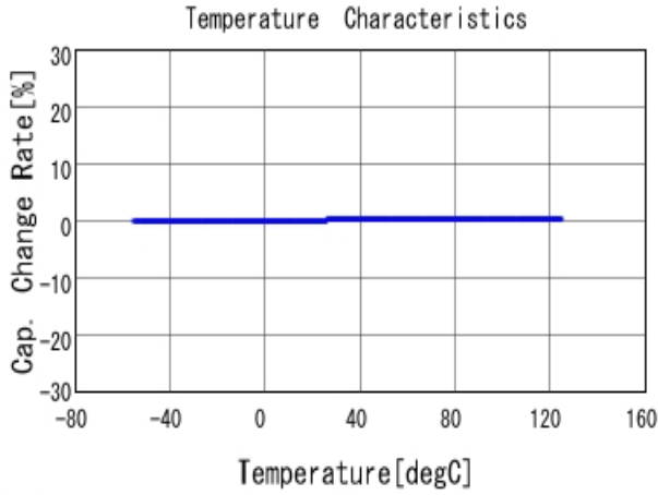
■ GRM31A5C3A820JW01 C-Temp. capchange, DCOV, AC1Vrms
