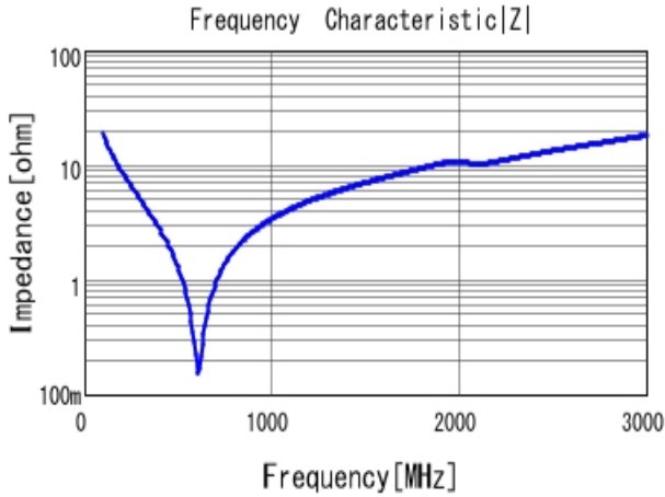
■ GRM31A5C3A820JW01 |Z| DC0V, 25degC
