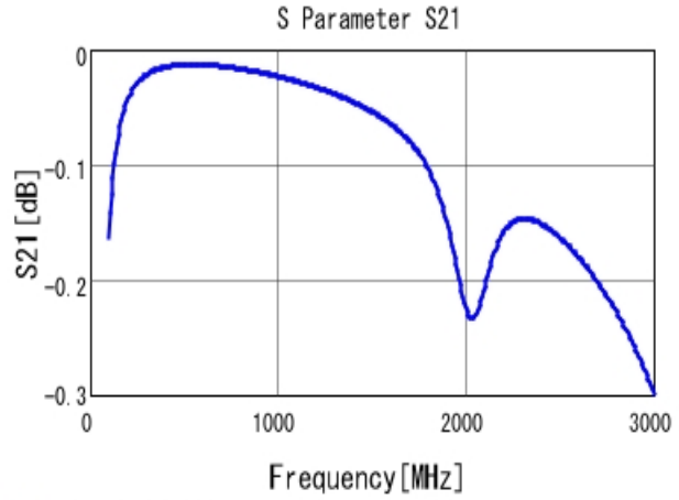
■ GRM31A5C3A820JW01 S21 DCOV, 25degC
