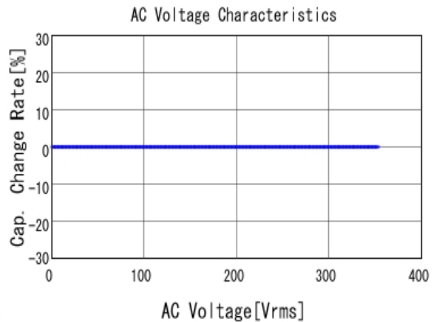
■ GRM31A5C3A820JW01 C-AC Voltage capchange, DC0V, 25.0d
