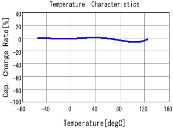
■ GRM15XR71H102KA86 C-Temp. capchange, DCO. 0V, AC1.0V rm
