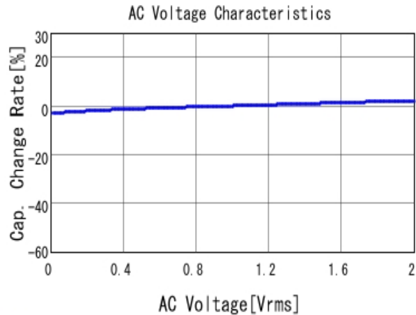
■ GRM15XR71H102KA86 C-AC Voltage capchange, DCOV, 25.0d
