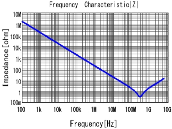
■ GRM15XR71H102KA86 |Z| DCOV, 25degC
