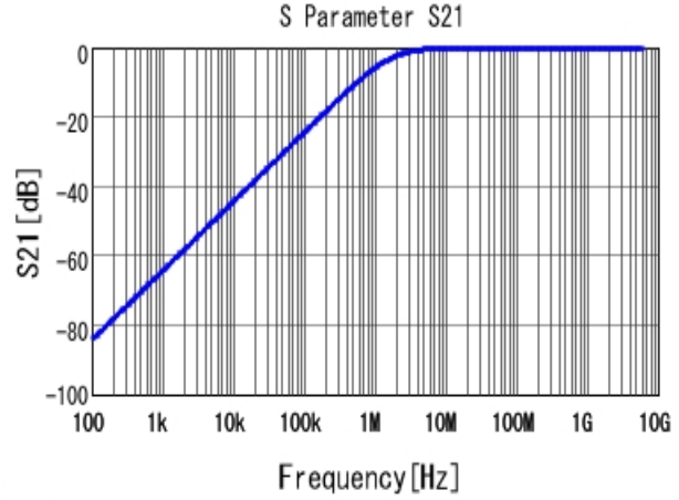
■ GRM15XR71H102KA86 S21 DCOV, 25degC
