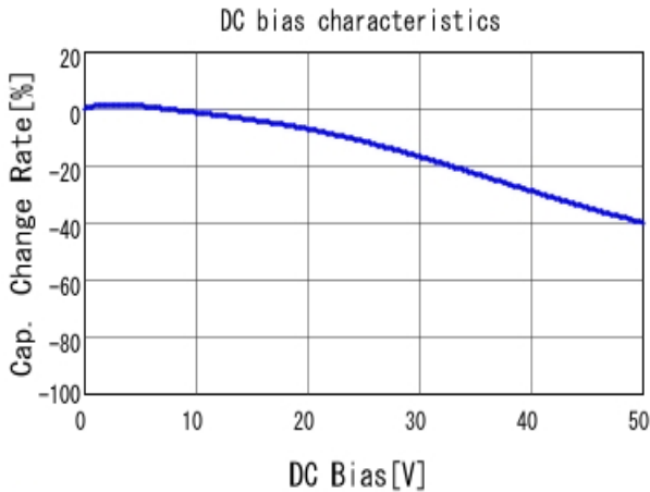
■ GRM15XR71H102KA86 C-DC bias capchange, 25.0degC, AC1.
