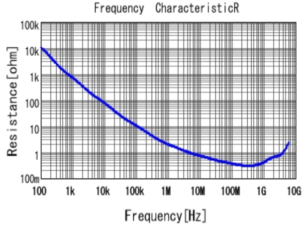
■ GRM15XR71H102KA86 R DCOV, 25degC
