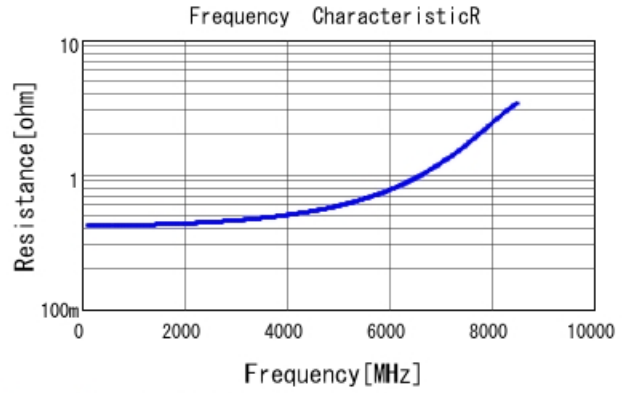
GRM1555C1H1R8BA01 R DCOV, 25degC
