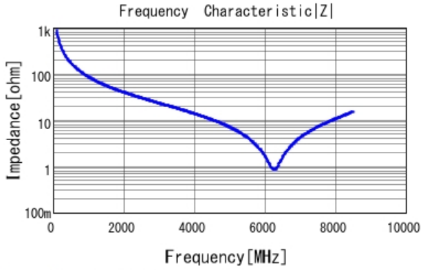
GRM1555C1H1R8BA01 |Z| DCOV, 25degC
