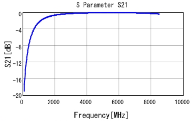
GRM1555C1H1R8BA01 S21 DCOV, 25degC
