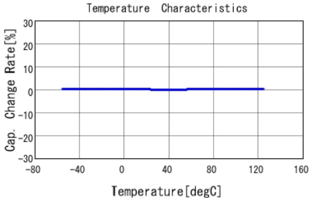
GRM1555C1H1R8BA01 C-Temp. capchange, DCOV, AC1Vrms
