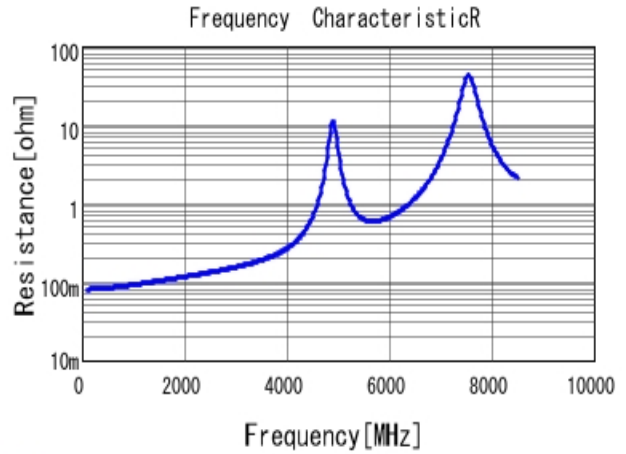
■ GJM1555C1H180FB01 R DC0V, 25degC
