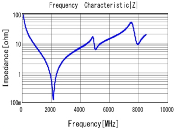
■ GJM1555C1H180FB01 |Z| DC0V, 25degC
