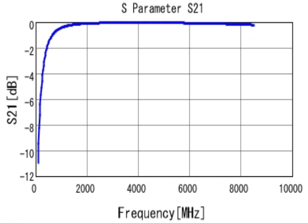
■ GRM0335C1H4R7BA01 S21 DCOV, 25degC
