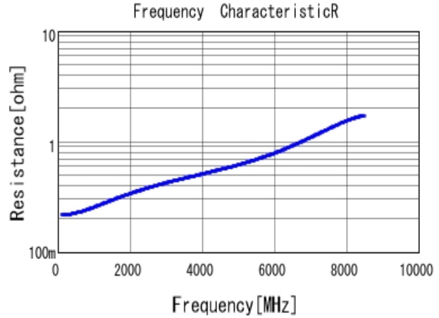
■ GRM0335C1H4R7BA01 R DC0V, 25degC
