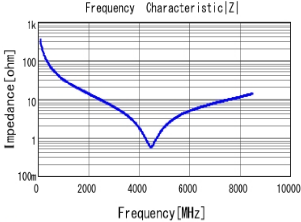
■ GRM0335C1H4R7BA01 |Z| DC0V, 25degC
