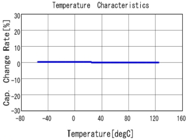
■ GRM0335C1H4R7BA01 C-Temp. capchange, DCOV, AC1Vrms
