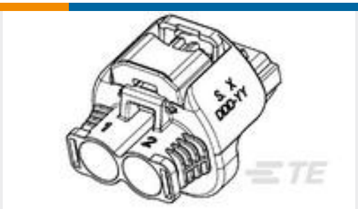
TE Part #1544978-3 RECEPT HSG ASSY, 8MM NG1+, 2W, SEALED
