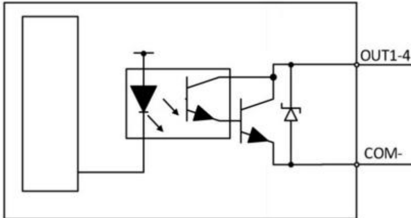
Figure 4-4 Output Schematic
