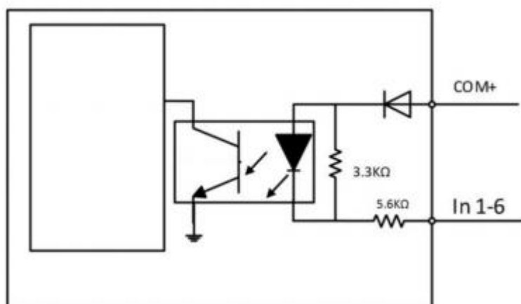
Figure 4-2 Input Schematic
