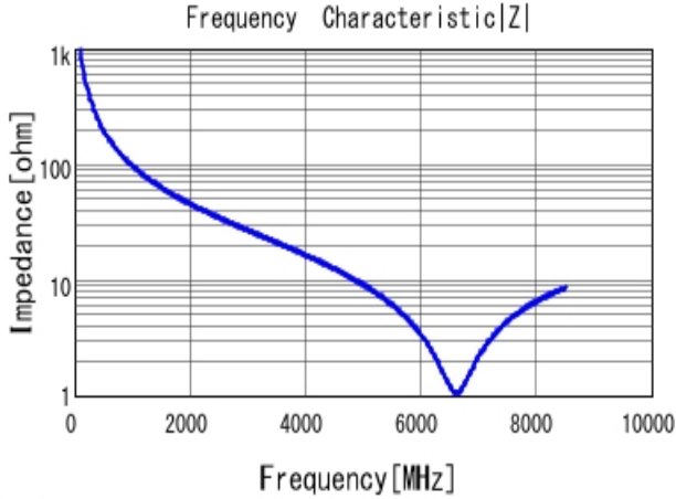
■ GRM1555C1H1R6CA01 |Z| DCOV, 25degC
