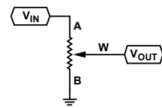
Figure 67. Potentiometer Mode Configuration
