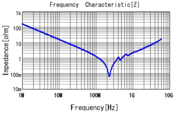
GCM1885C1H102JA16 |Z| DC0V, 25degC
