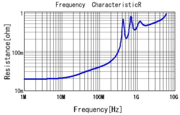
GCM1885C1H102JA16 R DC0V, 25degC
