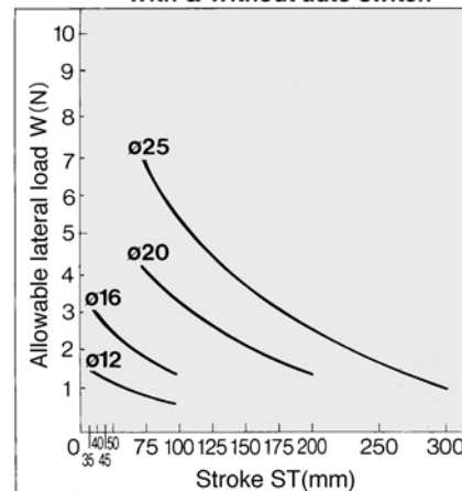
<Figure 5>Long stroke/ With & Without auto switch
