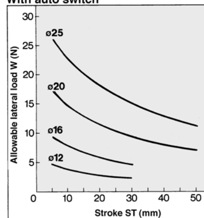
With auto switch
