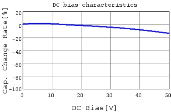
GCM188R71H472KA37 C-DC bias capchange, 25.0c
