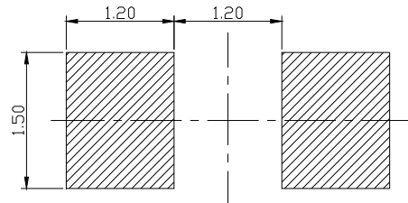
推荐焊盘尺寸 Recommended Soldering Pad
