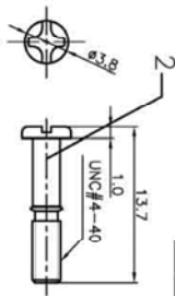
Short BOLT
