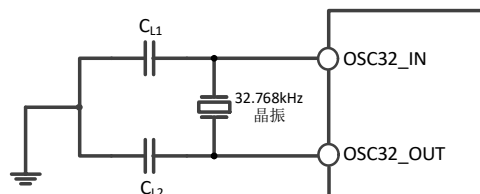
Figure 3-6 Typical Circuit of External 32.768K Crystal
