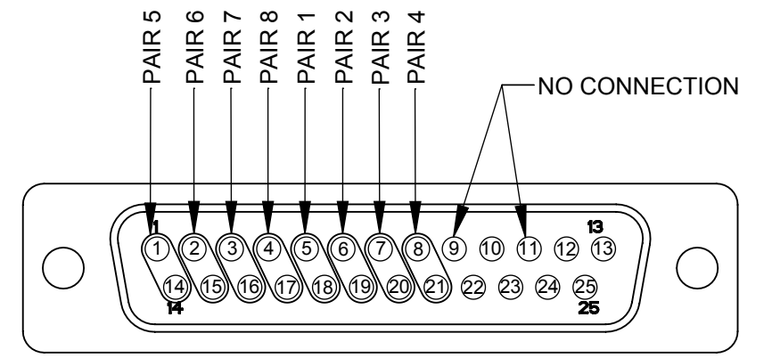
DB25 PIN-OUT VIEW
