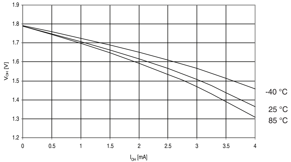
Figure 29-208. ATmega325PA: I/O Pin Output Voltage vs. Source Current, Ports A, C, D, E, F, G ( V_{CC} = 1.8V )
