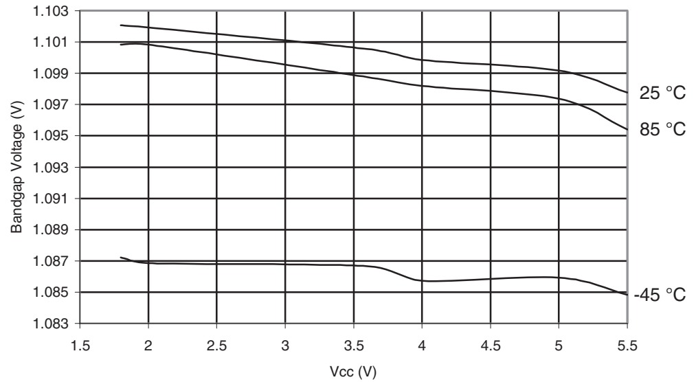
Figure 29-530. ATmega6450A: Bandgap Voltage vs. V CC
