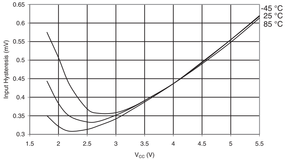
Figure 29-36. ATmega165A: I/O Pin Input Hysteresis vs. V_{CC}
