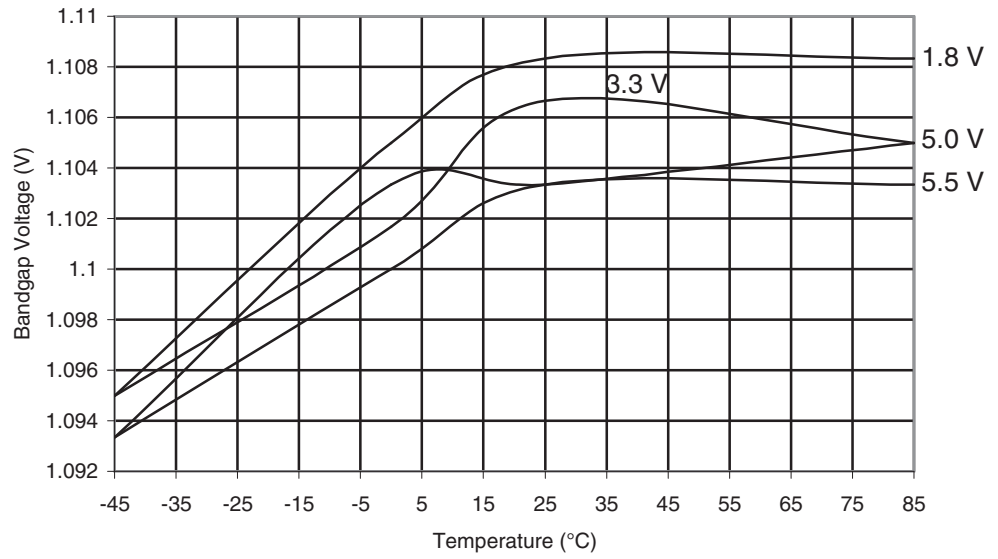
Figure 29-592. ATmega6450P: Bandgap Voltage vs. Temperature
