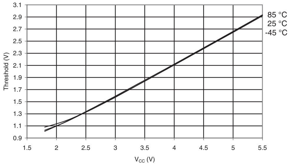
Figure 29-96. ATmega165PA: I/O Pin Input Threshold Voltage vs. V_{CC} ( V_{IH} , I/O Pin Read as “1”)
