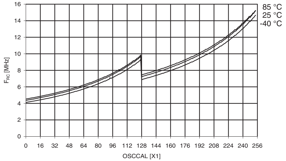
Figure 29-173. ATmega325A: Calibrated 8 MHz RC Oscillator Frequency vs. Oscal Value
