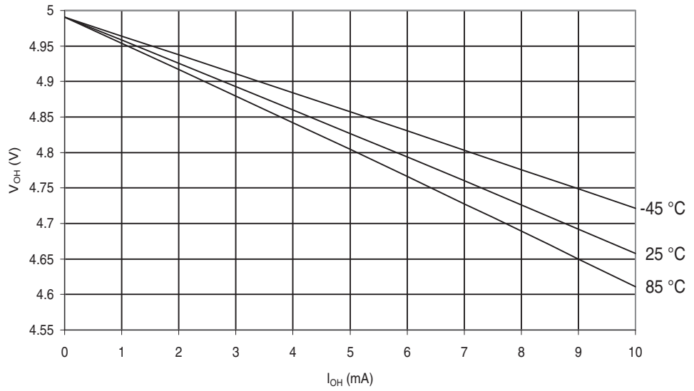
Figure 29-570. ATmega6450A: I/O Pin Output Voltage vs. Source Current, Ports A, C, D, E, F, G ( V_{CC} = 5V )
