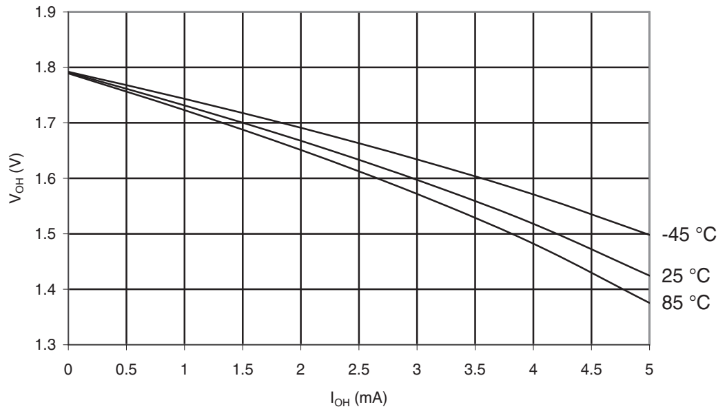
Figure 29-27. ATmega165A: I/O Pin Output Voltage vs. Source Current, Port B ( V_{CC} = 1.8V )
