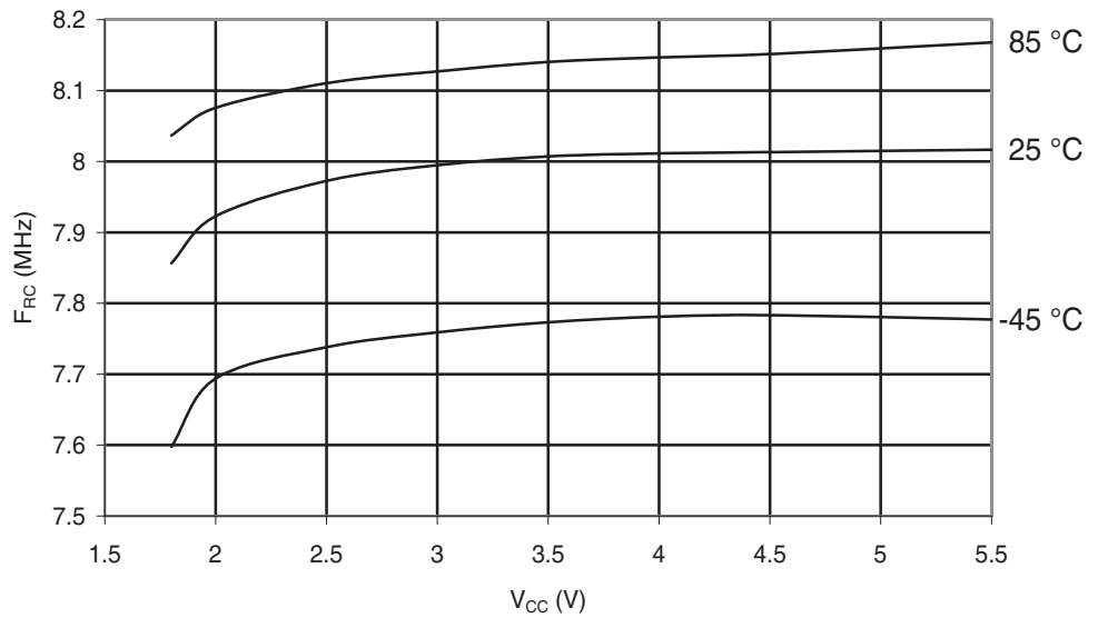
Figure 29-50. ATmega165A: Calibrated 8 MHz RC Oscillator Frequency vs. V_{CC}
