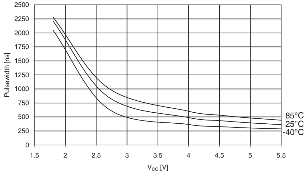
Figure 29-244. ATmega325PA: Minimum Reset Pulse Width vs. V_{CC}
