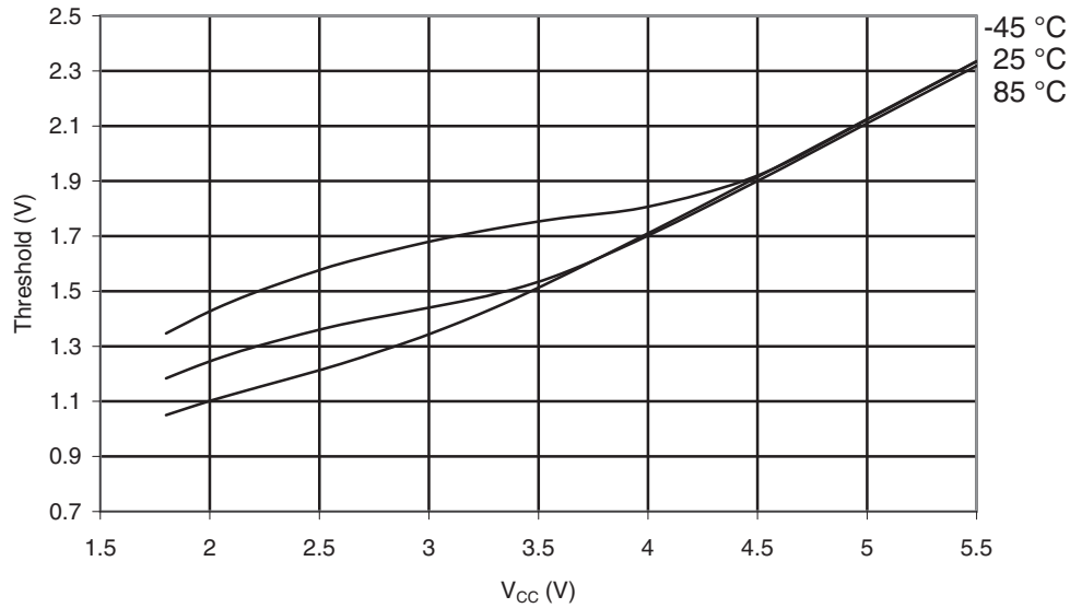
Figure 29-37. ATmega165A: Reset Input Threshold Voltage vs. V_{CC} ( V_{IH} , Reset Pin Read as “1”)
