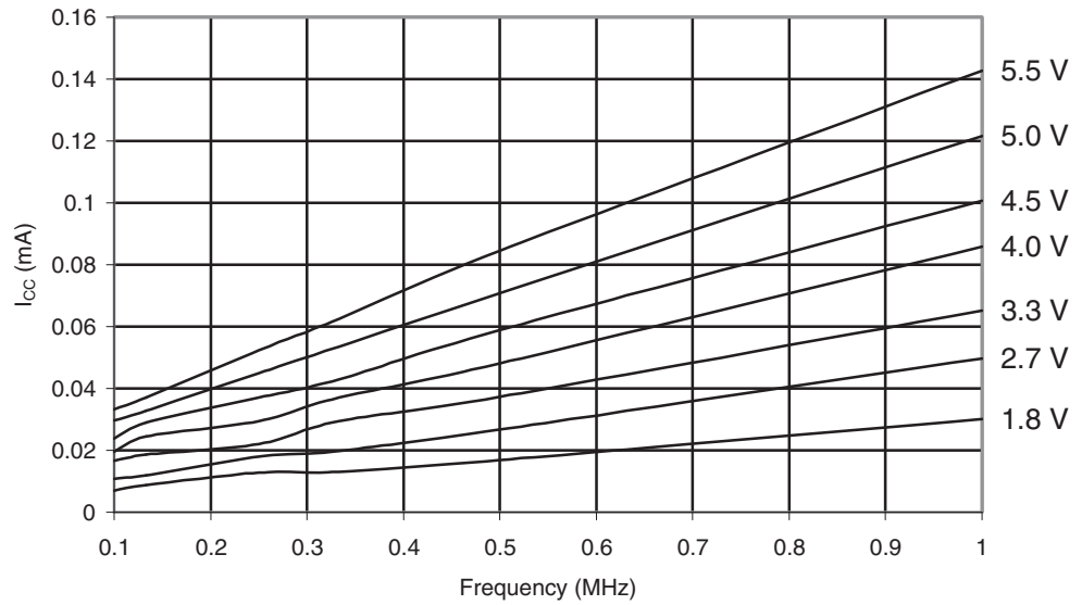
Figure 29-606. ATmega6450P: Reset Supply Current vs. V_{CC} (0.1 - 1.0 MHz, Excluding Current Through The Reset Pull-up)
