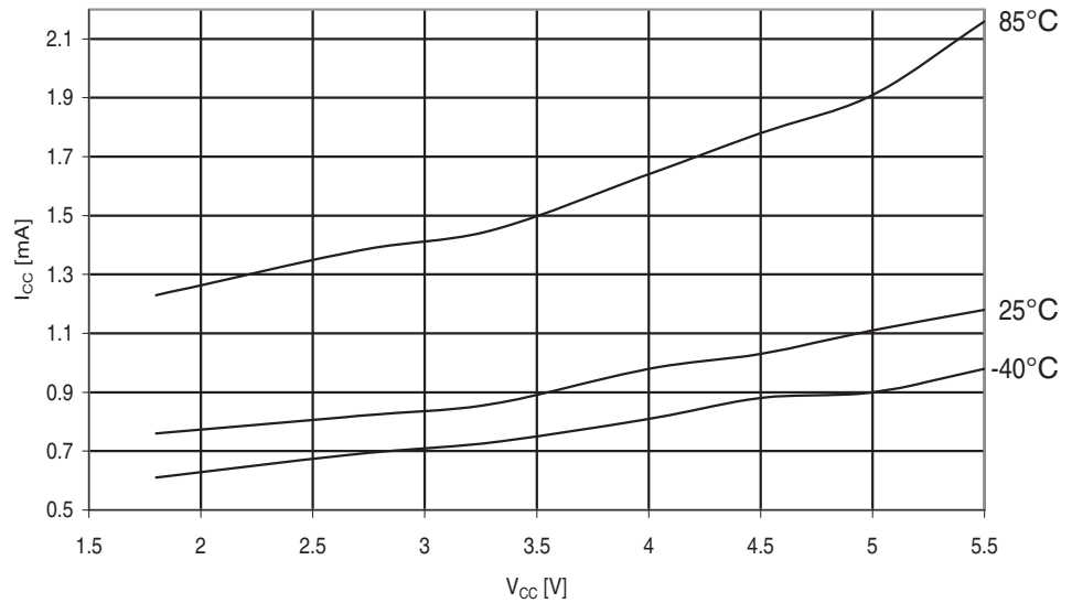
Figure 29-197. ATmega325PA: Power-save Supply Current vs. V_{CC} (Watchdog Timer Disabled and 32 kHz Crystal Oscillator Running)
