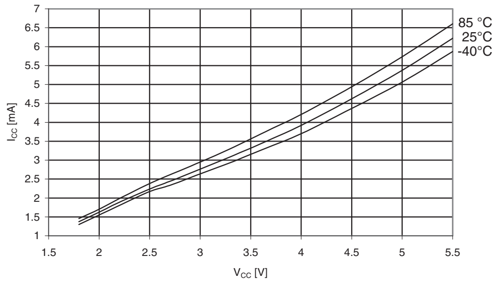
Figure 29-127. ATmega325A: Active Supply Current vs. V_{CC} (Internal RC Oscillator, 8 MHz)
