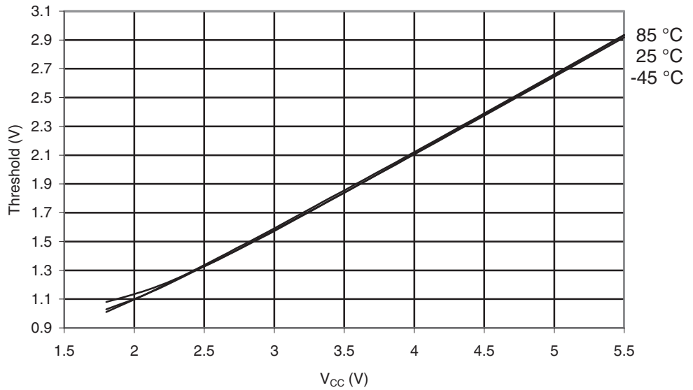
Figure 29-34. ATmega165A: I/O Pin Input Threshold Voltage vs. V_{CC} ( V_{IH} , I/O Pin Read as "1")
