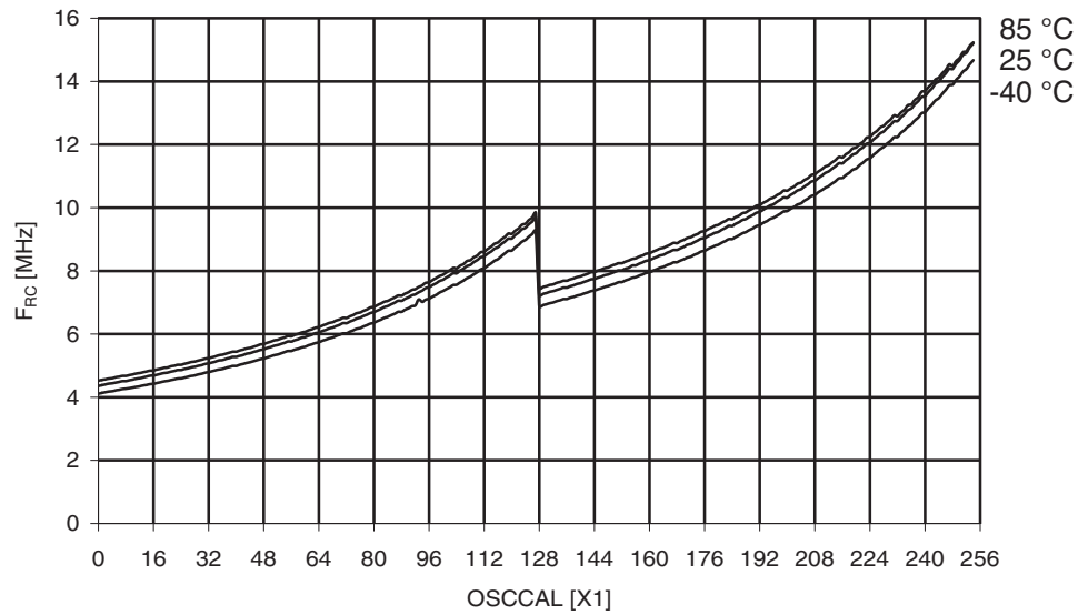
Figure 29-293. ATmega3250A: Calibrated 8 MHz RC Oscillator Frequency vs. Oscal Value
