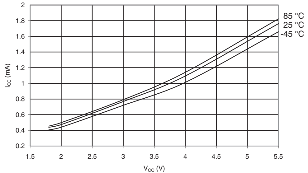
Figure 29-555. ATmega6450A: Idle Supply Current vs. V_{CC} (Internal RC Oscillator, 8 MHz)
