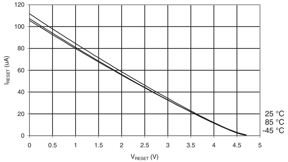
Figure 29-81. ATmega165PA: Reset Pull-up Resistor Current vs. Reset Pin Voltage ( V_{CC} = 5V )
