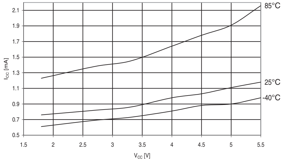
Figure 29-137. ATmega325A: Power-save Supply Current vs. V_{CC} (Watchdog Timer Disabled and 32 kHz Crystal Oscillator Running)
