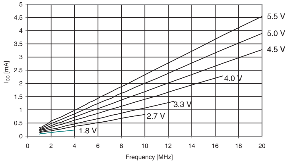
Figure 29-311. ATmega3250PA: Idle Supply Current vs. Frequency (1 - 20 MHz)
