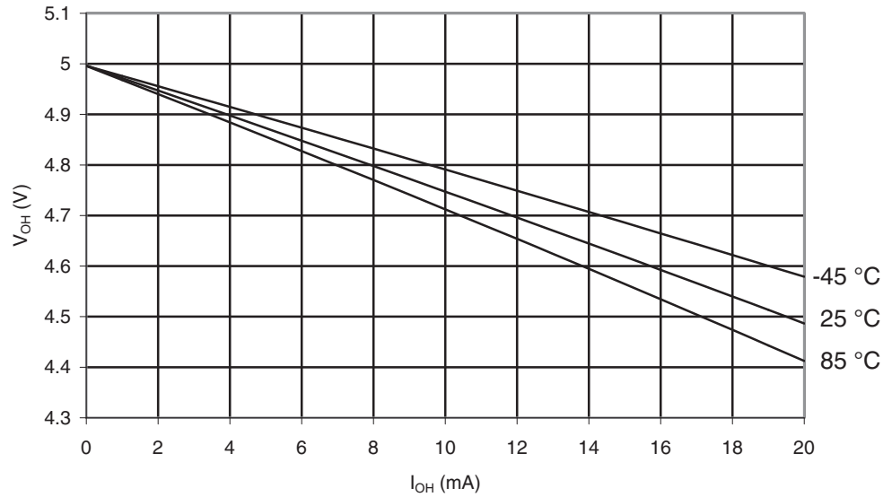
Figure 29-25. ATmega165A: I/O Pin Output Voltage vs. Source Current, Port B ( V_{CC} = 5V )
