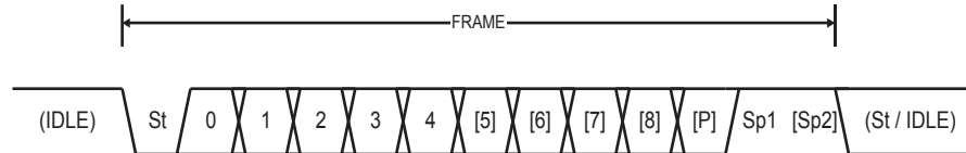
Figure 19-4. Frame Formats
