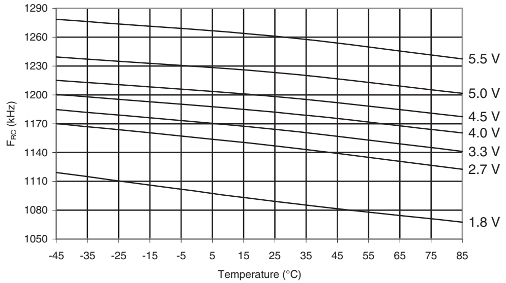
Figure 29-472. ATmega645P: Watchdog Oscillator Frequency vs. Temperature
