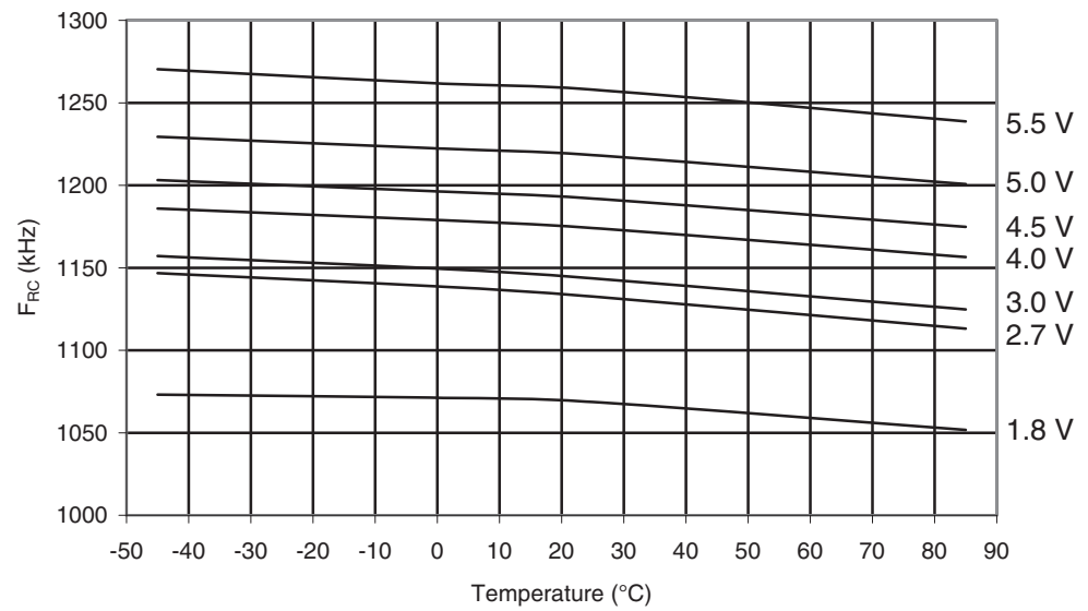
Figure 29-110. ATmega165PA: Watchdog Oscillator Frequency vs. Temperature
