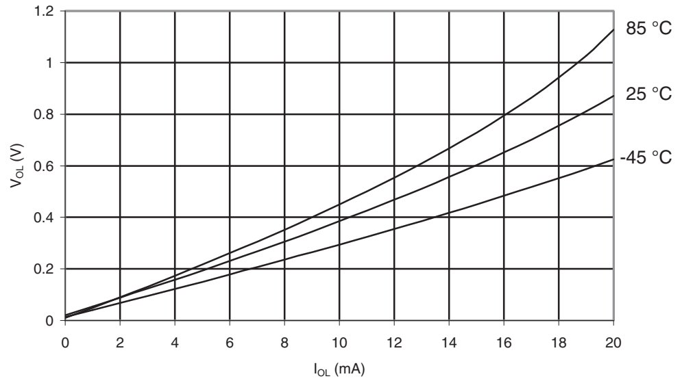
Figure 29-580. ATmega6450P: I/O Pin Output Voltage vs. Sink Current, Port B ( V_{CC} = 2.7V_9 )
