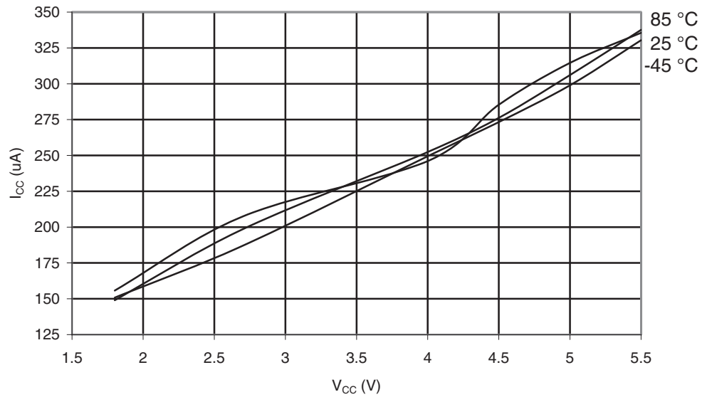
Figure 29-117. ATmega165A: Active Supply Current with ADC at 1 MHz vs. V_{CC}
