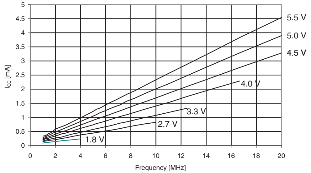
Figure 29-191. ATmega325PA: Idle Supply Current vs. Frequency (1 - 20 MHz)
