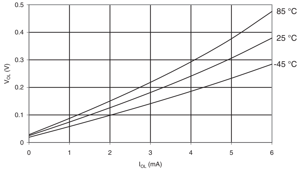
Figure 29-95. ATmega165PA: I/O Pin Output Voltage vs. Sink Current, Port B ( V_{CC} = 1.8V )
