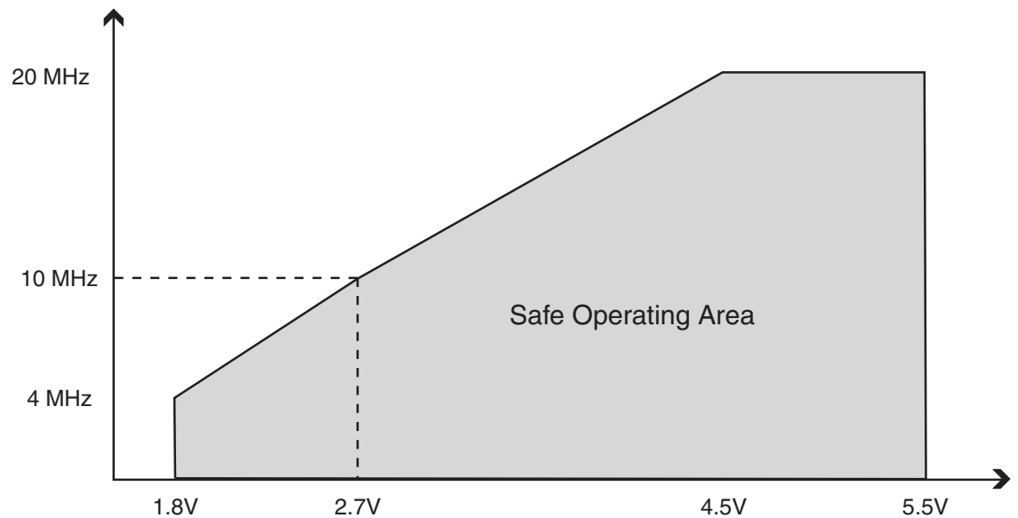
Figure 27-2. Maximum Frequency vs. V_{CC} (10 - 20 MHz) ATmega325A/ATmega325PA/ATmega3250A/ATmega3250PA/ATmega6450A/ ATmega6450P
