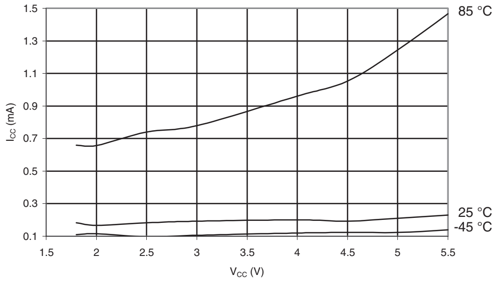
Figure 29-377. ATmega645A: Power-down Supply Current vs. V_{CC} (32 kHz Watch Crystal)
