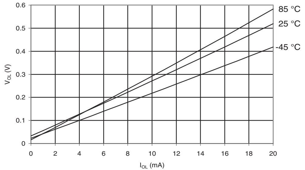
Figure 29-518. ATmega6450A: I/O Pin Output Voltage vs. Sink Current, Port B ( V_{CC} = 5V )
