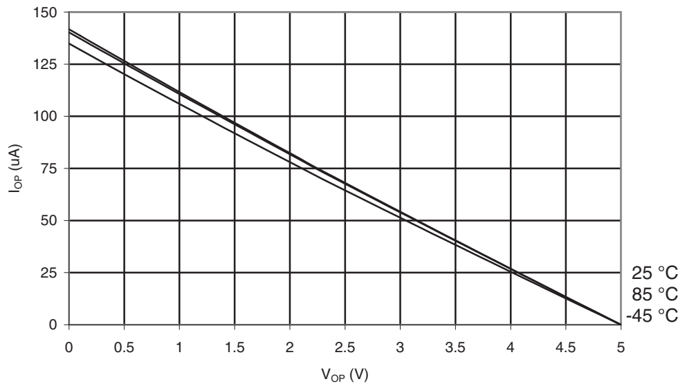
Figure 29-78. ATmega165PA: I/O Pin Pull-up Resistor Current vs. Input Voltage ( V_{CC} = 5V )
