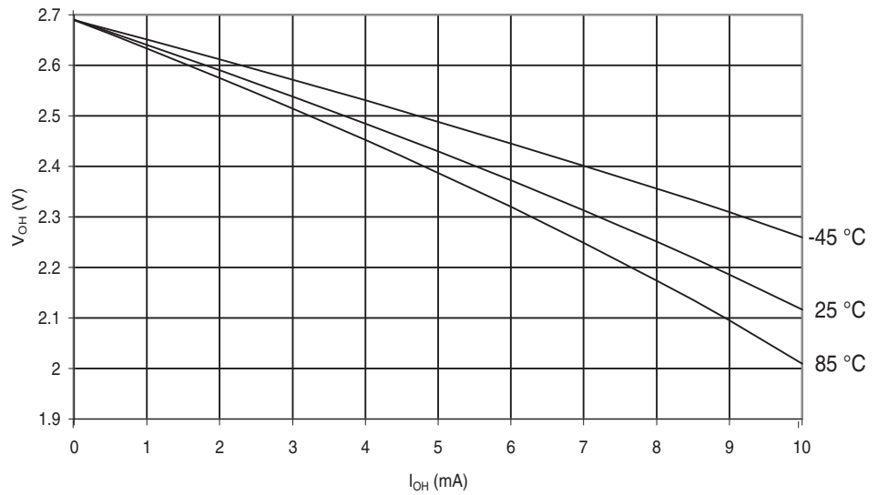
Figure 29-571. ATmega6450A: I/O Pin Output Voltage vs. Source Current, Ports A, C, D, E, F, G ( V_{CC} = 2.7V )
