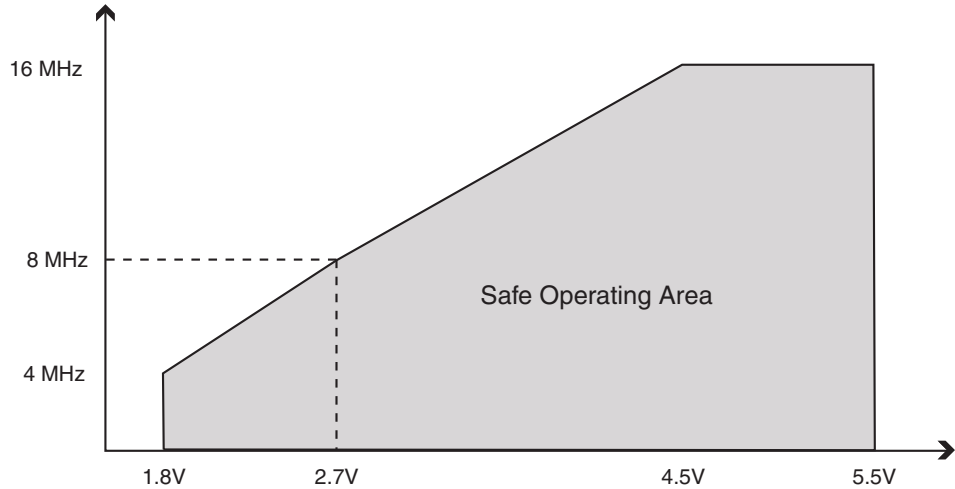
Figure 27-1. Maximum Frequency vs. V_{CC} : ATmega165A/165PA/ATmega645A/ATmega645P
