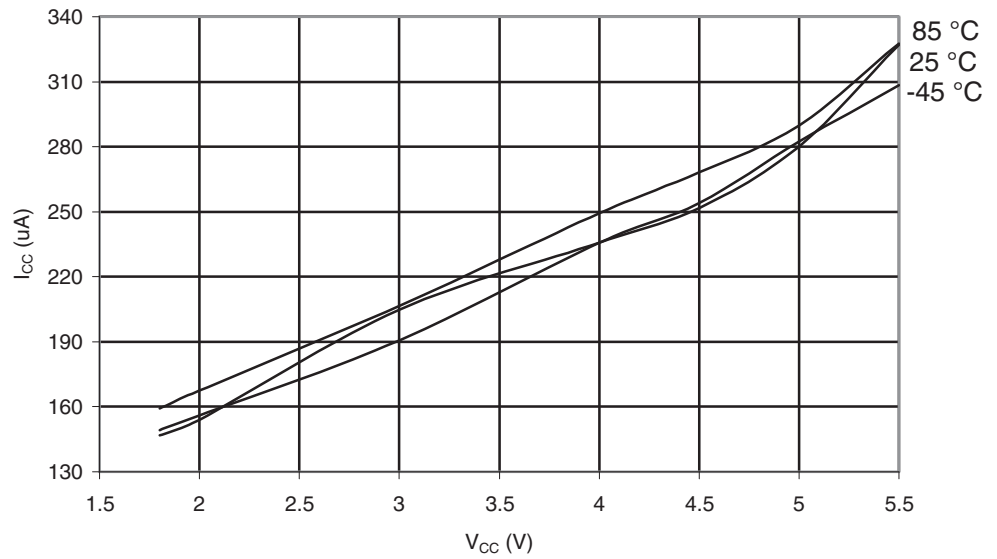
Figure 29-601. ATmega6450P: Active Supply Current with ADC at 1 MHz vs. V_{CC}
