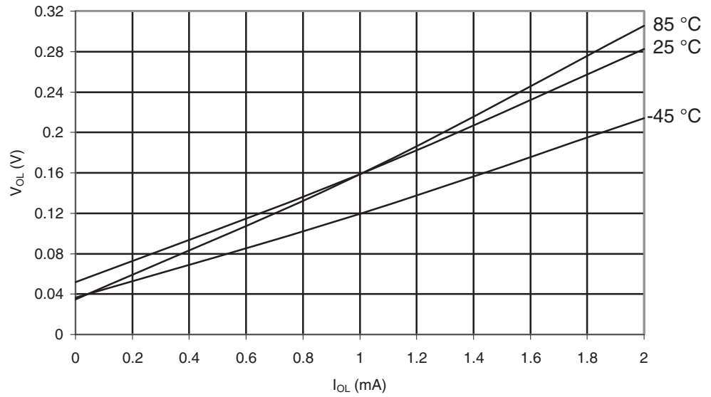
Figure 29-517. ATmega6450A: I/O Pin Output Voltage vs. Sink Current, Ports A, C, D, E, F, G ( V_{CC} = 1.8V )
