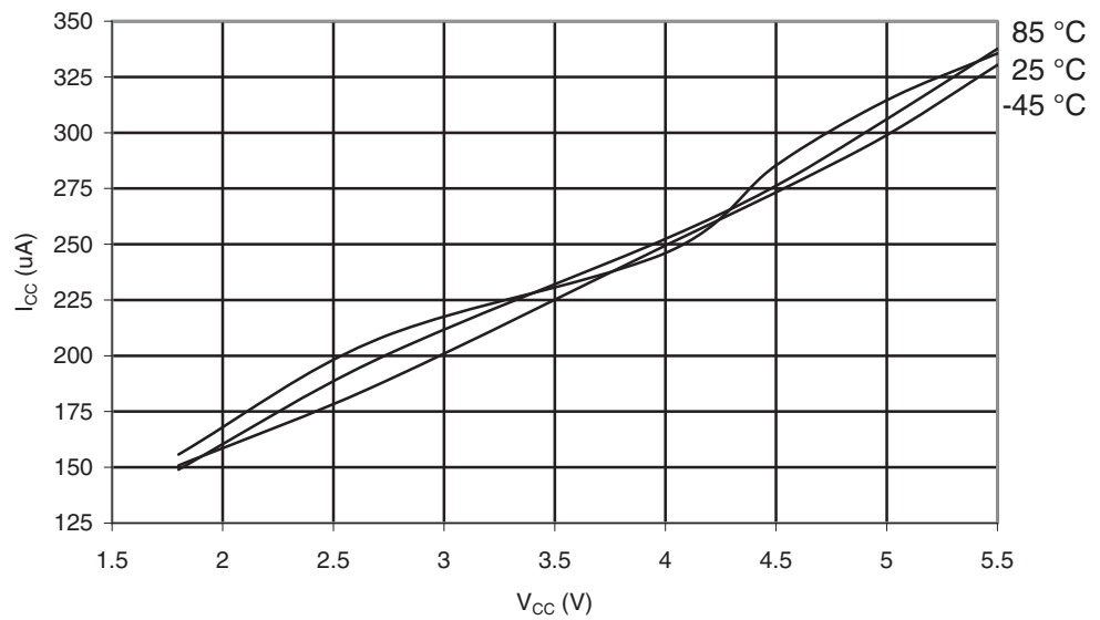
Figure 29-55. ATmega165A: Active Supply Current with ADC at 1 MHz vs. V_{CC}
