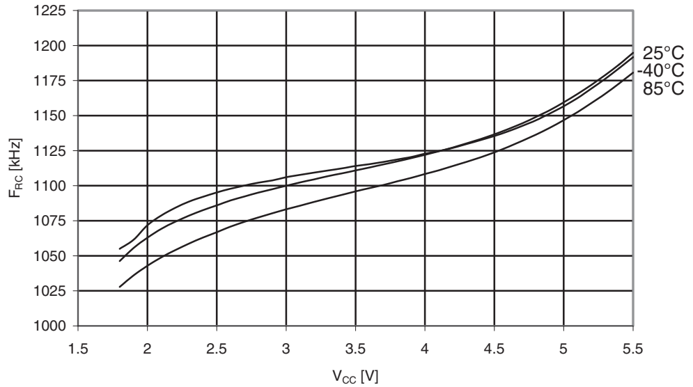
Figure 29-169. ATmega325A: Watchdog Oscillator Frequency vs. V_{CC}
