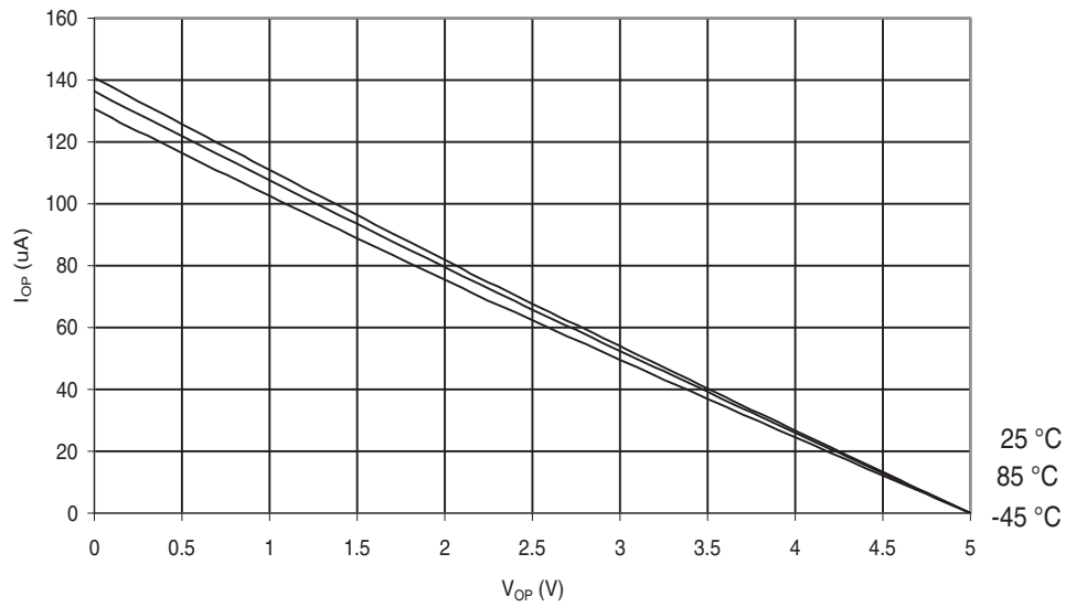
Figure 29-442. ATmega645P: I/O Pin Pull-up Resistor Current vs. Input Voltage ( V_{CC} = 5V )
