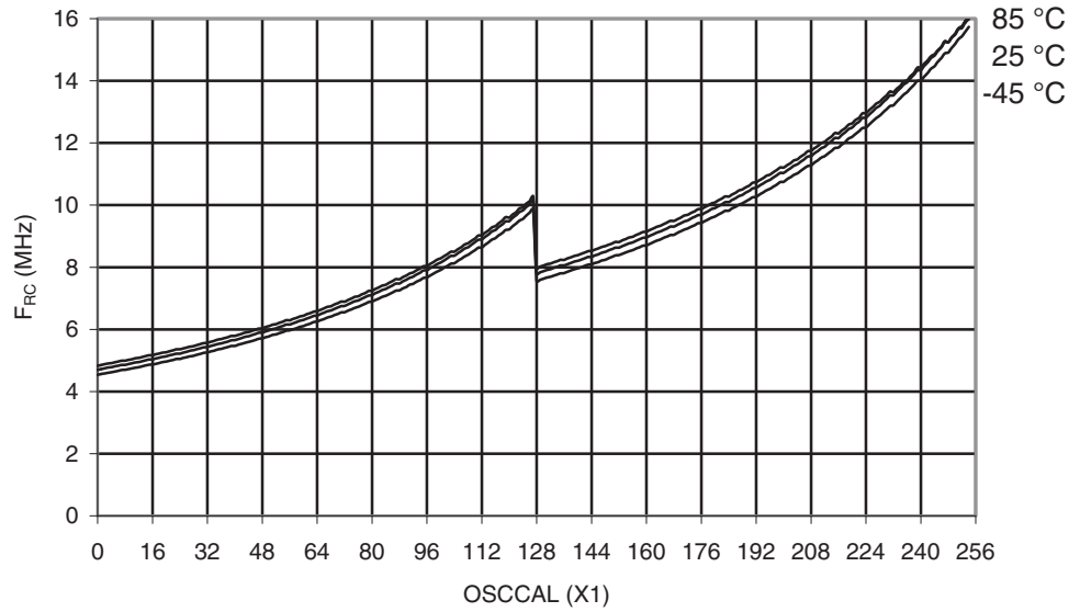
Figure 29-113. ATmega165PA: Calibrated 8 MHz RC Oscillator Frequency vs. Oscal Value
