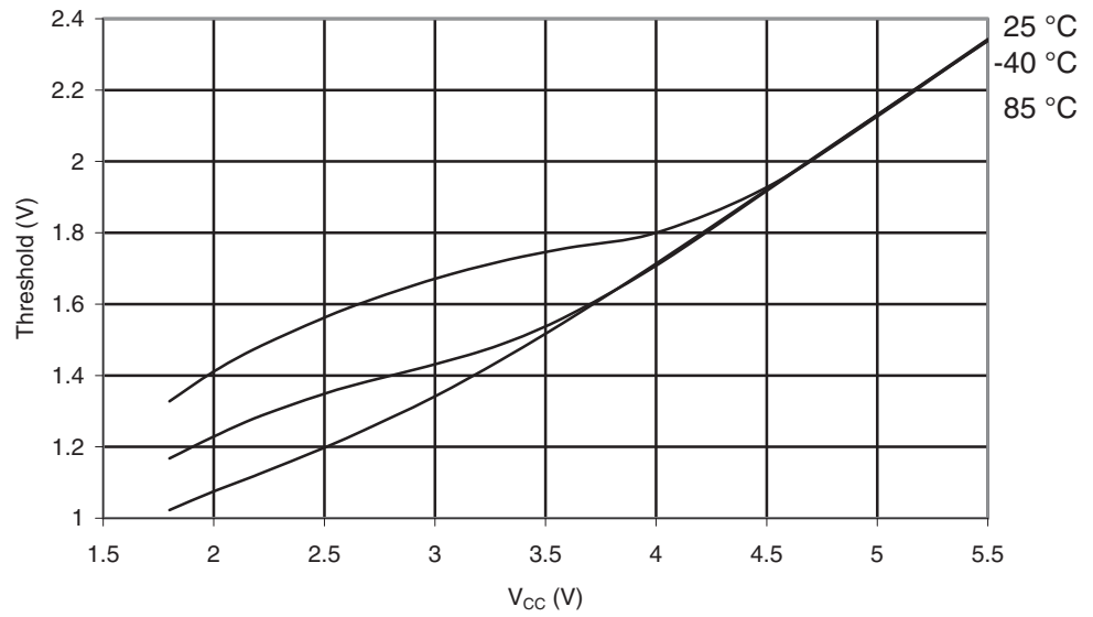
Figure 29-281. ATmega3250A: Reset Input Threshold Voltage vs. V_{CC} ( V_{IH} , Reset Pin Read as "1")
