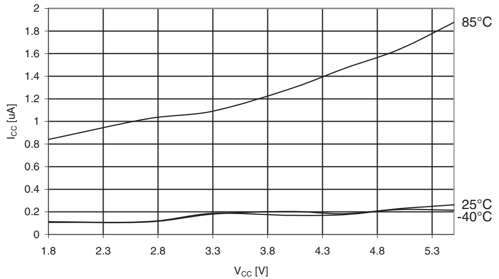
Figure 29-255. ATmega3250A: Power-down Supply Current vs. V_{CC} (Watchdog Timer Disabled)
