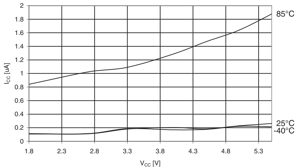
Figure 29-315. ATmega3250PA: Power-down Supply Current vs. V_{CC} (Watchdog Timer Disabled)
