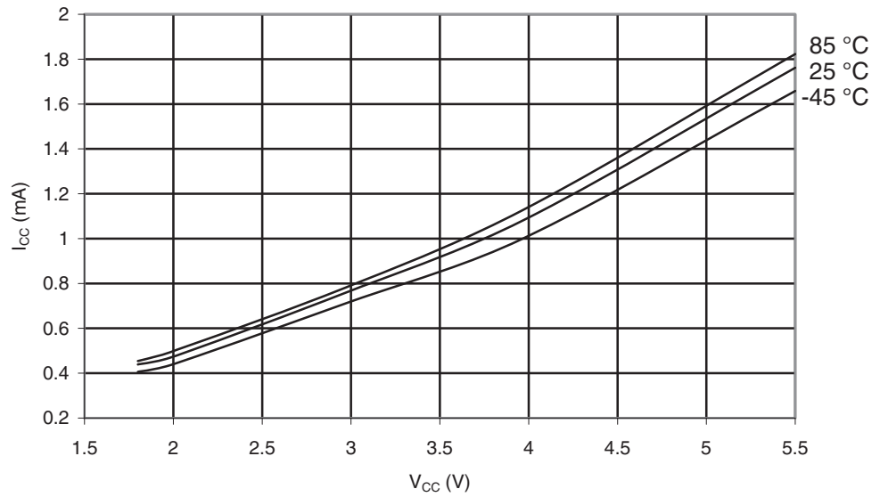
Figure 29-433. ATmega645P: Idle Supply Current vs. V_{CC} (Internal RC Oscillator, 8 MHz)
