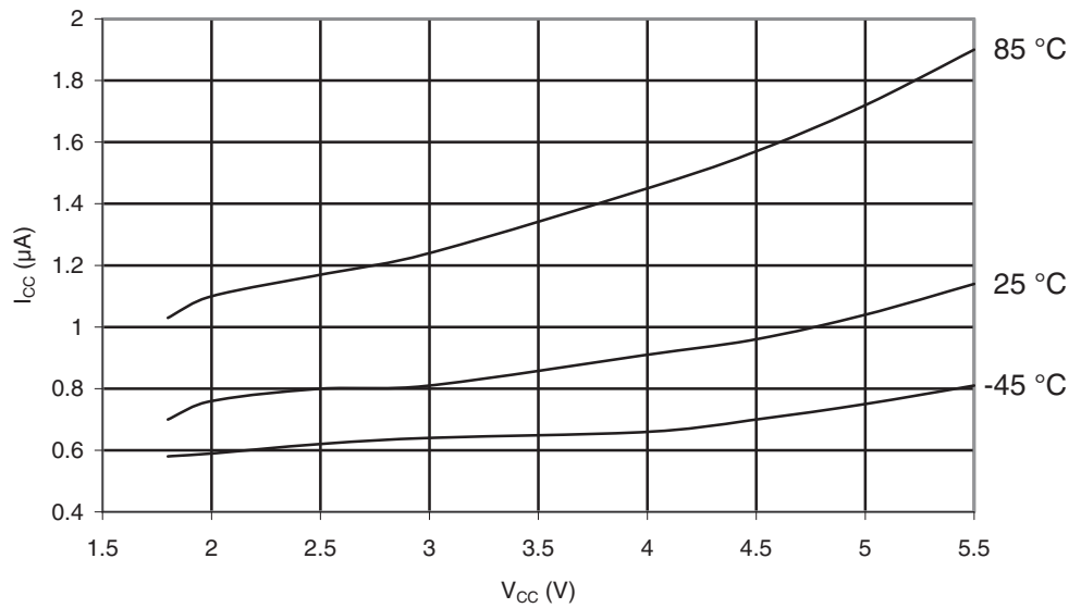
Figure 29-75. ATmega165PA: Power-save Supply Current vs. V_{CC} (Watchdog Timer Disabled)
