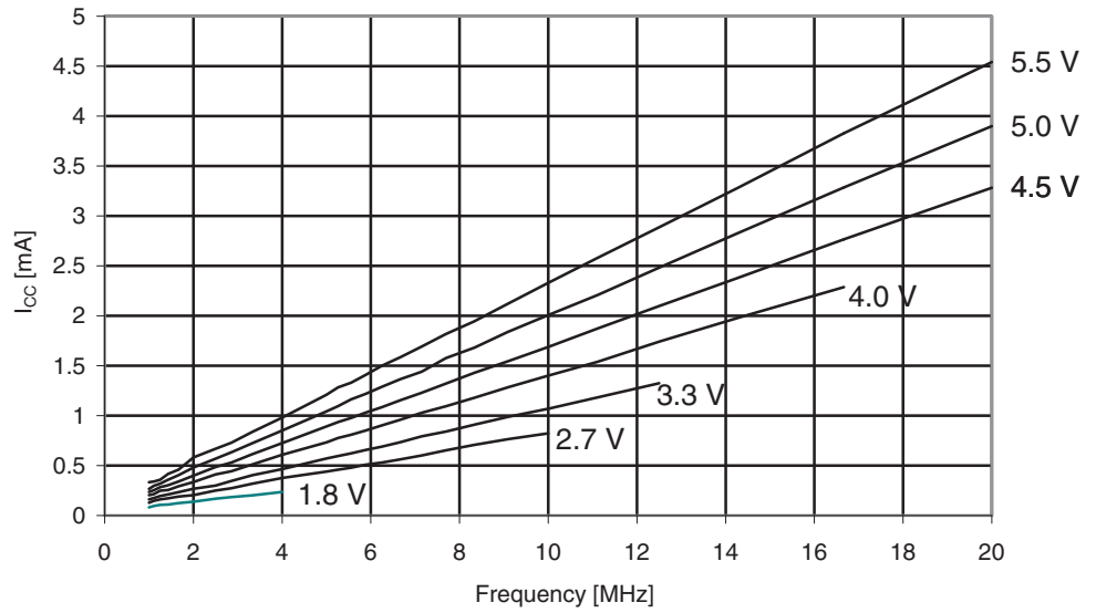
Figure 29-251. ATmega3250A: Idle Supply Current vs. Frequency (1 - 20 MHz)
