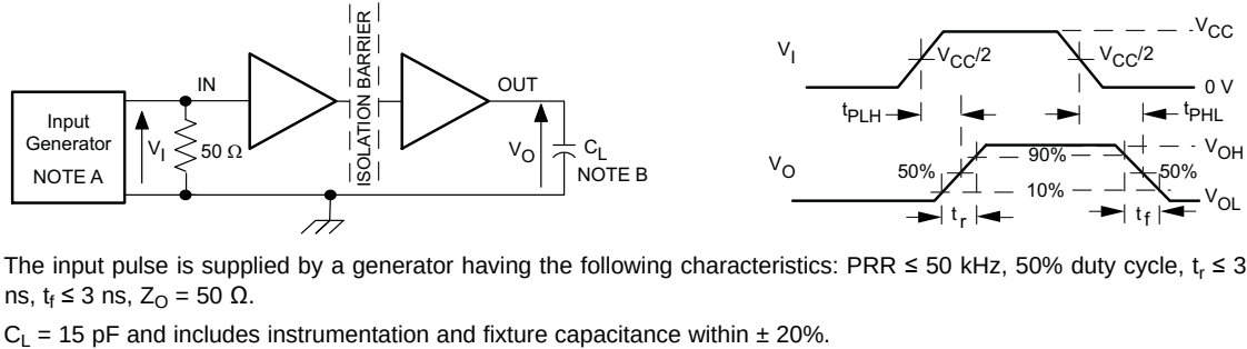
Figure 13. Switching Characteristic Test Circuit and Voltage Waveforms
