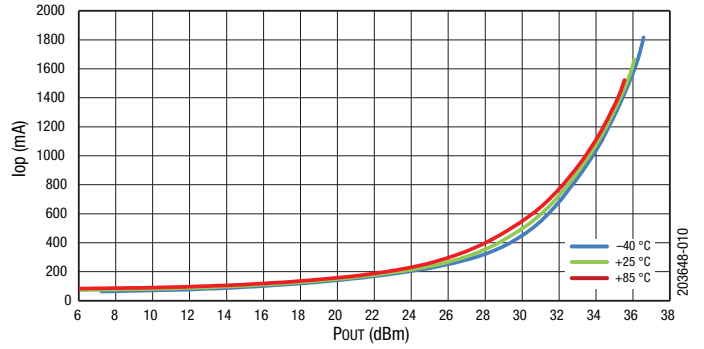
Figure 10. Operating Current vs POUT Across Temperature
