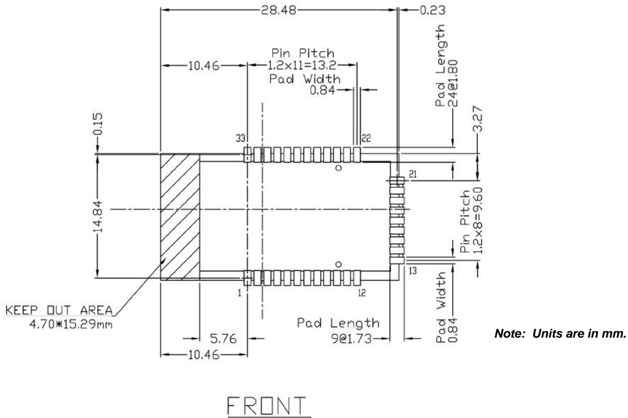
Figure 10: PCB Land Pattern and Antenna Keep-out for BT730-SA
