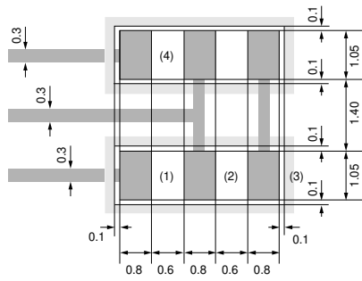
(1) : Input (2) : Ground (3) : Float Signal Line (4) : Out put [Shaded Area] It shows solder resist land pattern.
