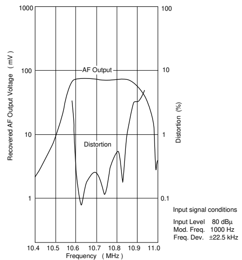
Frequency Characteristics
