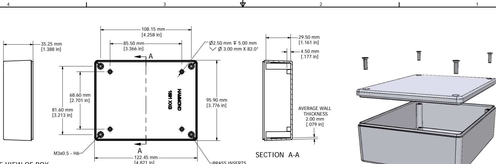
SIDE VIEW OF BOX
