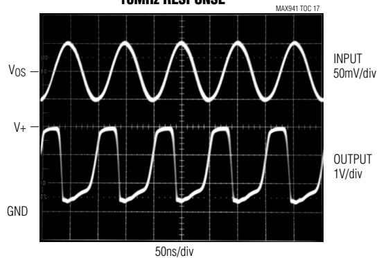
10MHz RESPONSE
