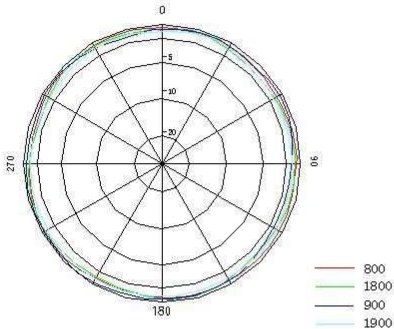
Vertical Pattern
