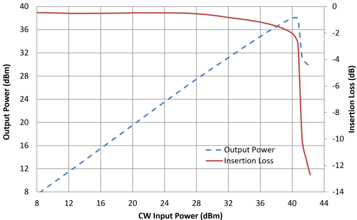
Figure 2. Output Power and Insertion Loss vs Input Power (f = 2.3 GHz)
