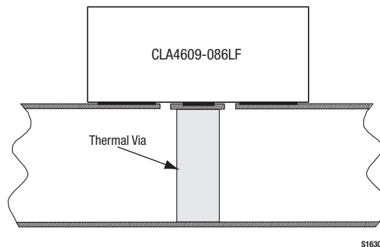
Figure 5. Cross-Sectional View of Suggested Printed Circuit Board
