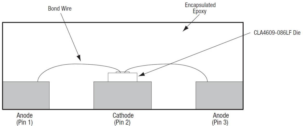
Figure 6. Cross-Sectional View of the CLA4609-086LF
