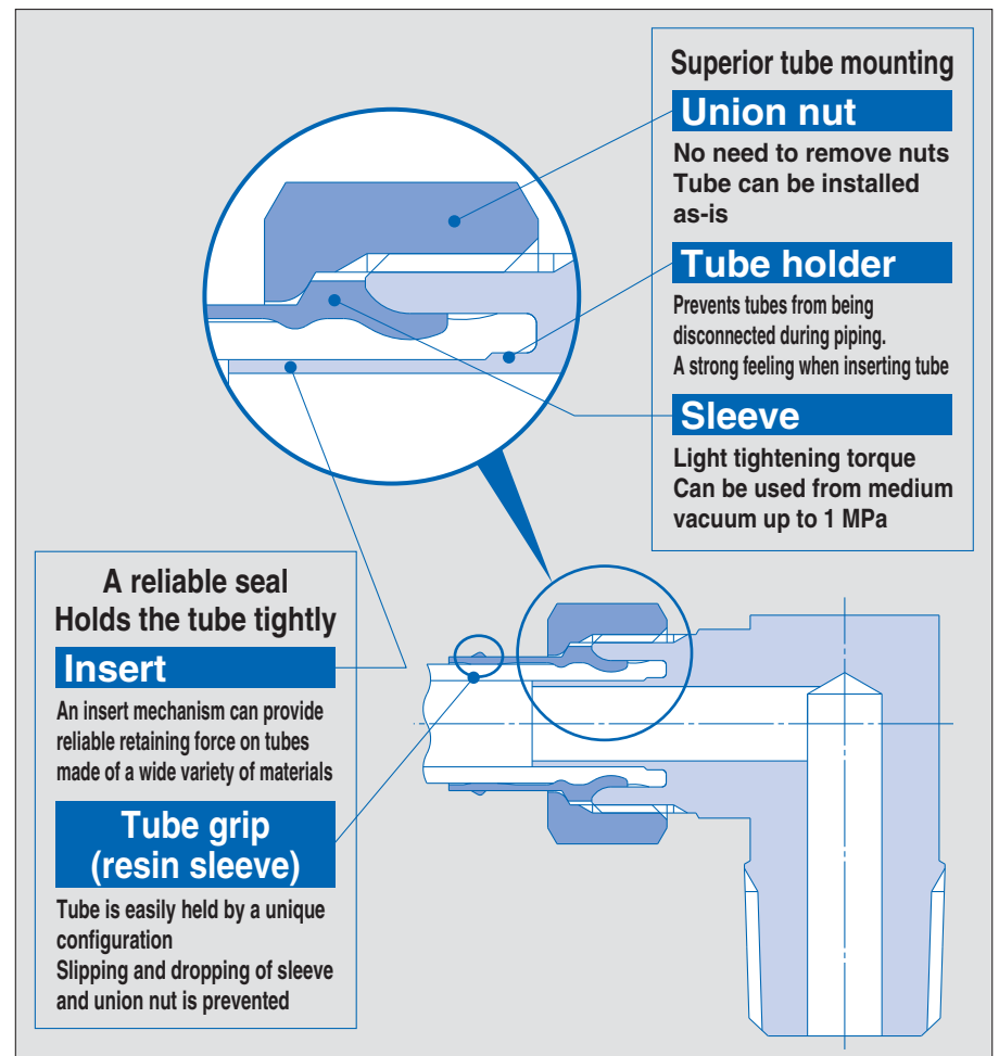
Resin sleeve
