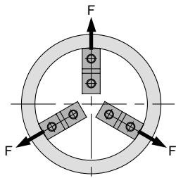
Internal gripping
