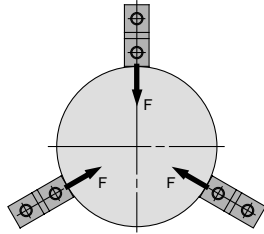
External gripping
