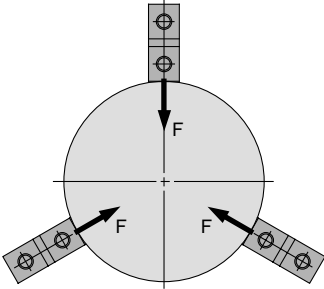
External gripping
