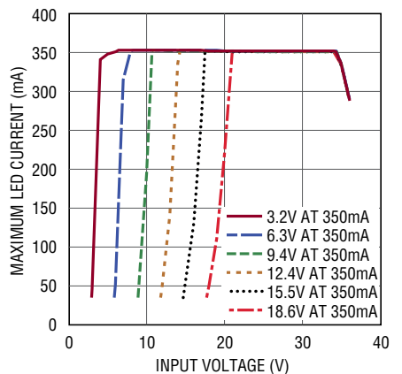
Maximum LED Current vs Input Voltage, Buck Mode
