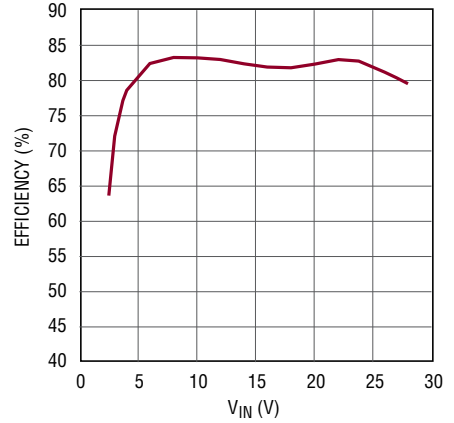
Efficiency vs V_{IN} , Buck-Boost Mode, 6.7V at 350mA LED String
